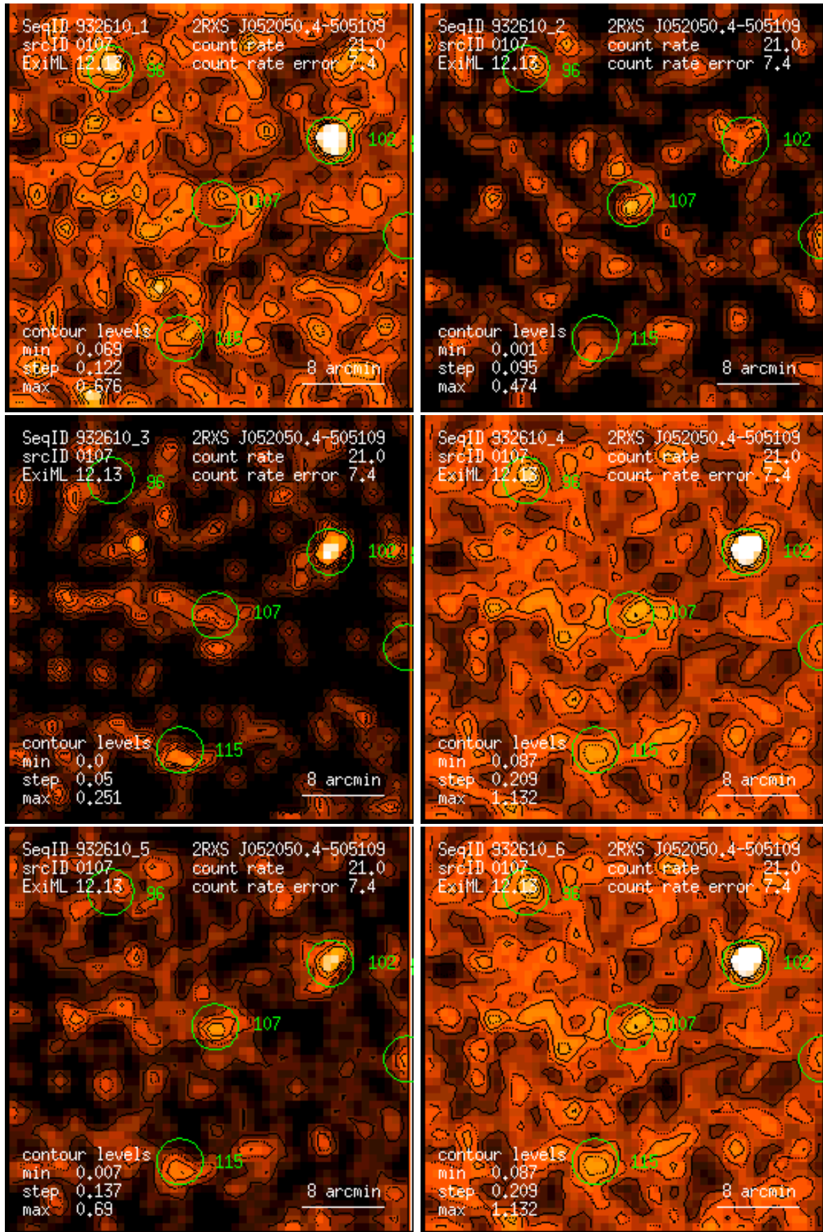
Figure 107: RASS 932610: detection 0107: band rate images, Gaussian filter: (1) PSPC channels 11 – 41, (2) 52 – 90, (3) 91 – 201, (4) 11 – 235, (5) 52 – 201, (6) 11 – 201. Broad band rates in counts/ks. Band rate contour levels in counts/ks/arcmin 2 .
