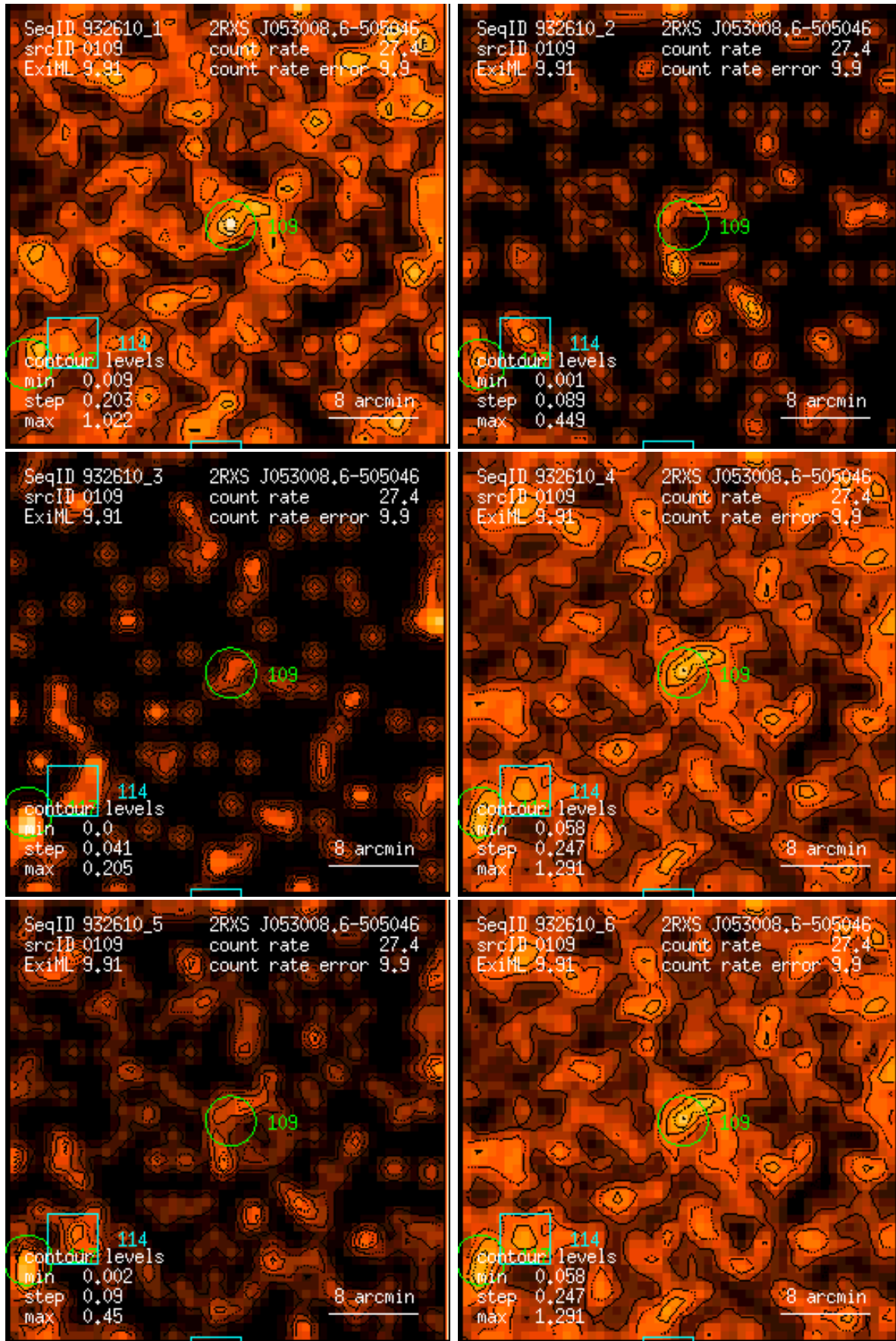
Figure 109: RASS 932610: detection 0109: band rate images, Gaussian filter: (1) PSPC channels 11 – 41, (2) 52 – 90, (3) 91 – 201, (4) 11 – 235, (5) 52 – 201, (6) 11 – 201. Broad band rates in counts/ks. Band rate contour levels in counts/ks/arcmin 2 .
