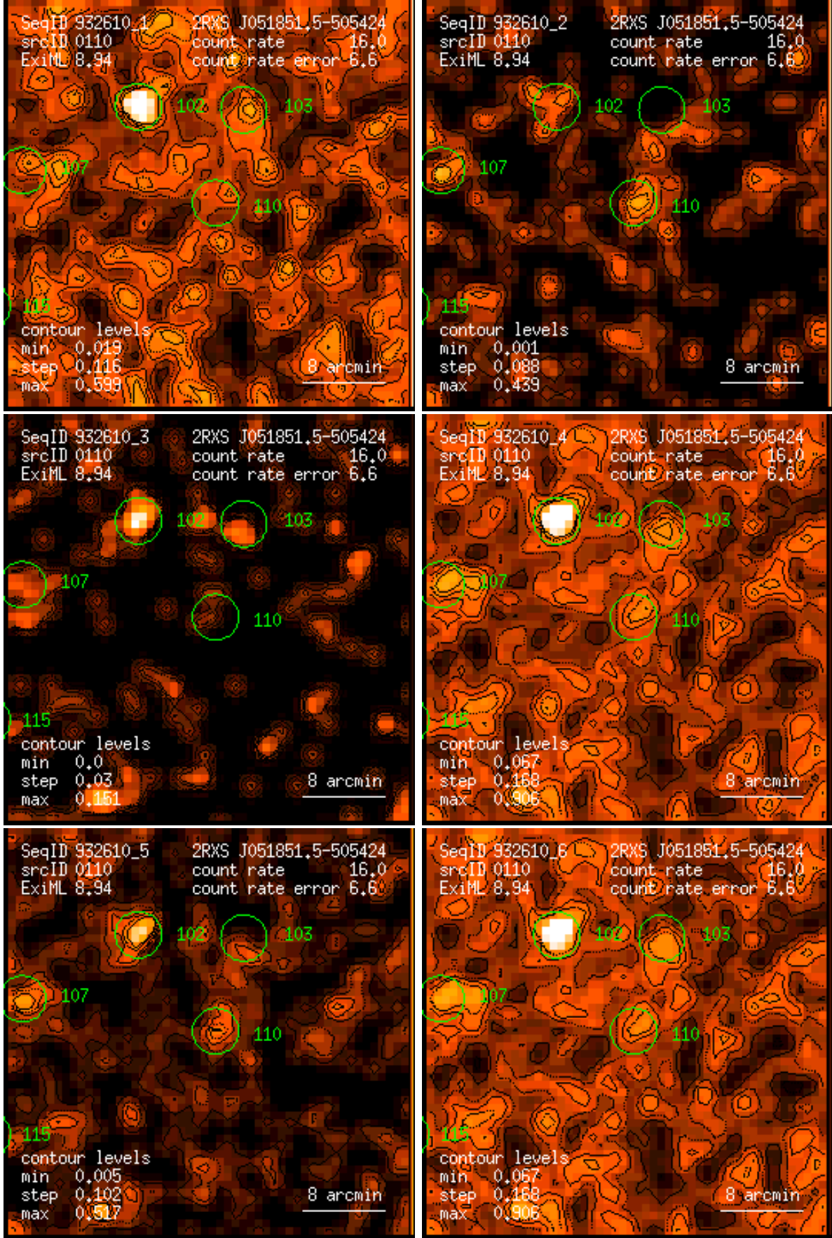
Figure 110: RASS 932610: detection 0110: band rate images, Gaussian filter: (1) PSPC channels 11 – 41, (2) 52 – 90, (3) 91 – 201, (4) 11 – 235, (5) 52 – 201, (6) 11 – 201. Broad band rates in counts/ks. Band rate contour levels in counts/ks/arcmin 2 .
