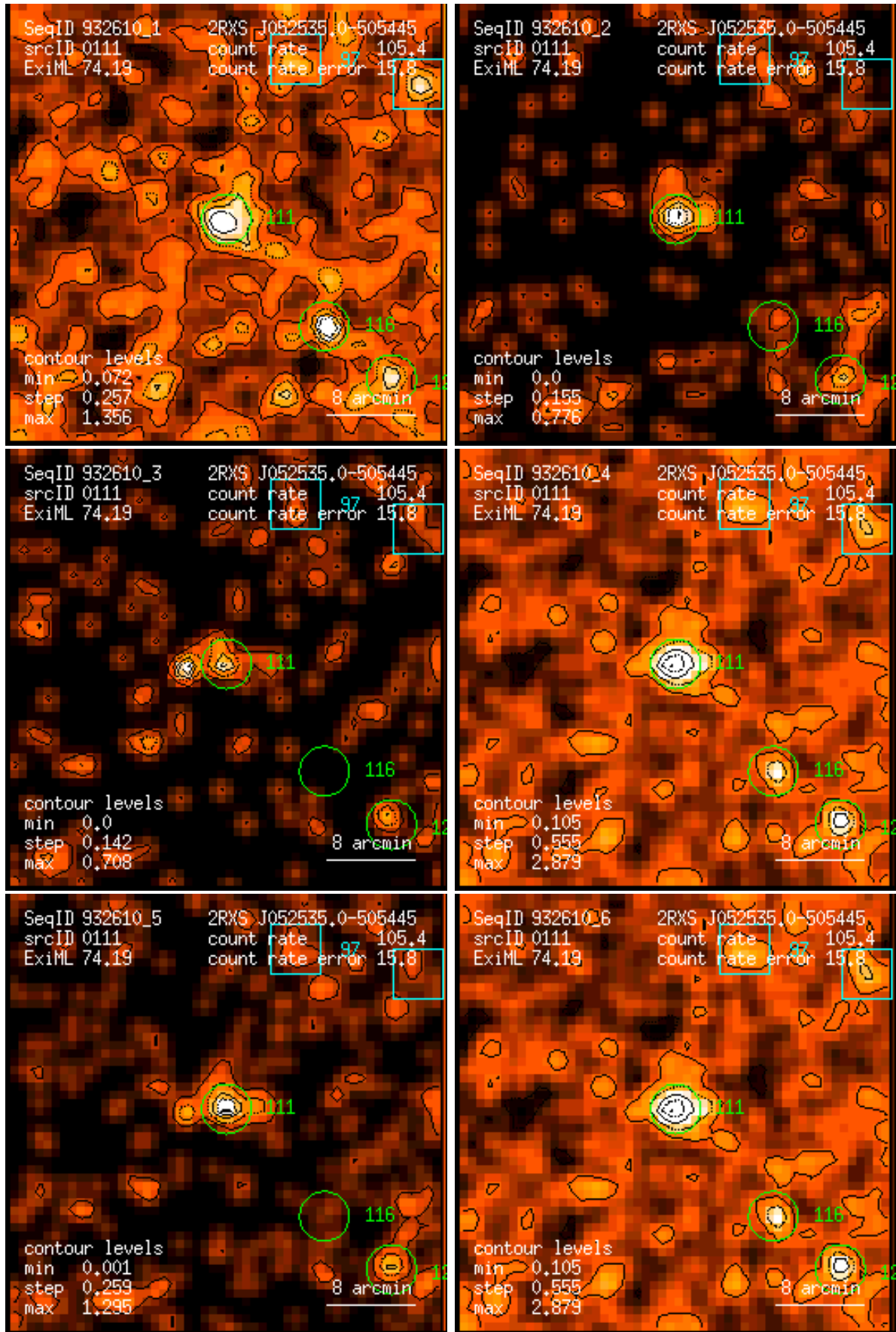
Figure 111: RASS 932610: detection 0111: band rate images, Gaussian filter: (1) PSPC channels 11 – 41, (2) 52 – 90, (3) 91 – 201, (4) 11 – 235, (5) 52 – 201, (6) 11 – 201. Broad band rates in counts/ks. Band rate contour levels in counts/ks/arcmin 2 .
