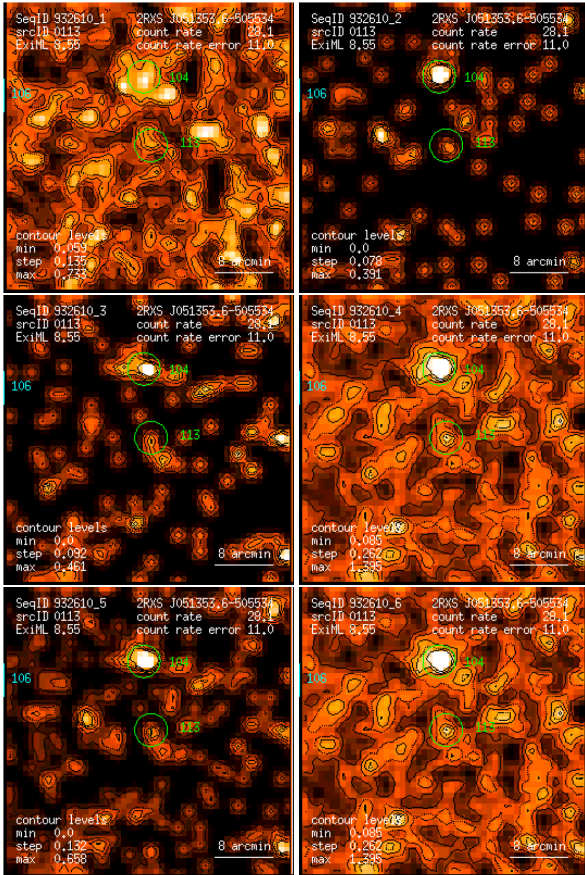
Figure 113: RASS 932610: detection 0113: band rate images, Gaussian filter: (1) PSPPC channels 11 – 41, (2) 52 – 90, (3) 91 – 201, (4) 11 – 235, (5) 52 – 201, (6) 11 – 201. Broad band rates in counts/ks. Band rate contour levels in counts/ks/arcmin 2 .
