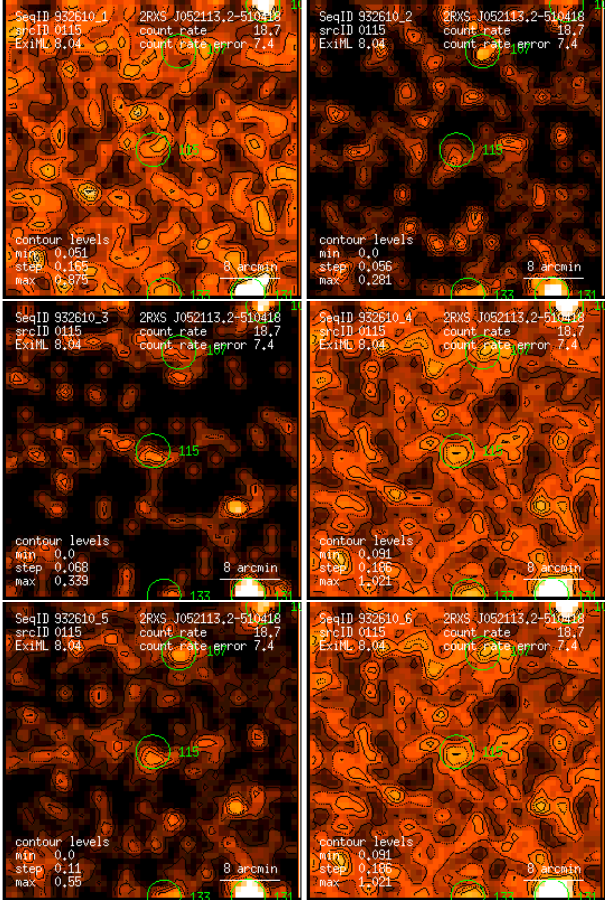
Figure 115: RASS 932610: detection 0115: band rate images, Gaussian filter: (1) PSPC channels 11 – 41, (2) 52 – 90, (3) 91 – 201, (4) 11 – 235, (5) 52 – 201, (6) 11 – 201. Broad band rates in counts/ks. Band rate contour levels in counts/ks/arcmin 2 .
