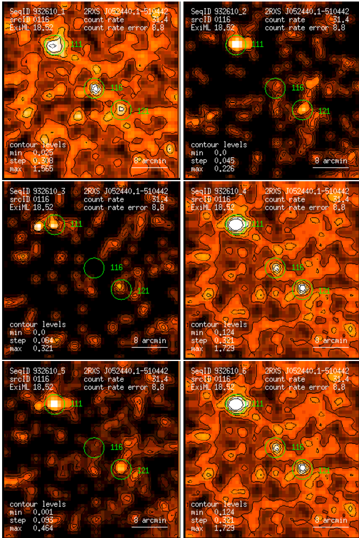
Figure 116: RASS 932610: detection 0116: band rate images, Gaussian filter: (1) PSPC channels 11 – 41, (2) 52 – 90, (3) 91 – 201, (4) 11 – 235, (5) 52 – 201, (6) 11 – 201. Broad band rates in counts/ks. Band rate contour levels in counts/ks/arcmin 2 .
