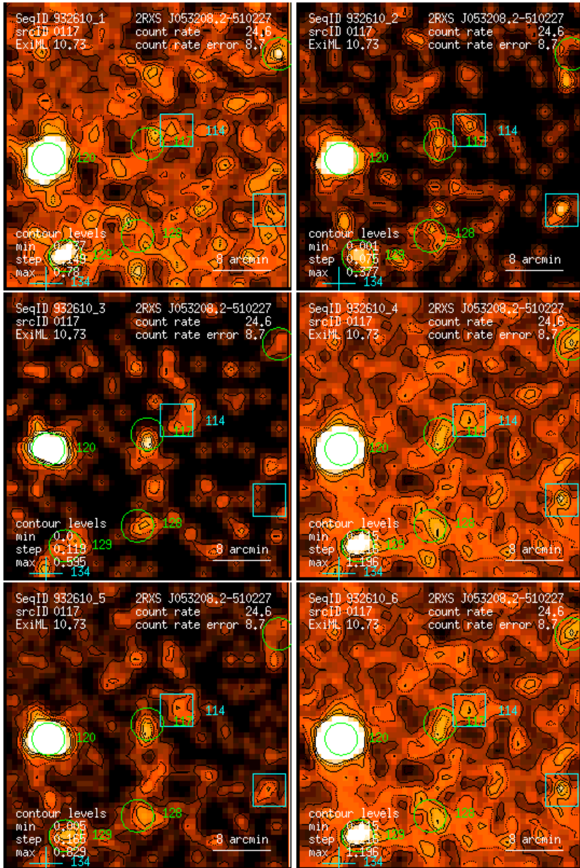
Figure 117: RASS 932610: detection 0117: band rate images, Gaussian filter: (1) PSPC channels 11 – 41, (2) 52 – 90, (3) 91 – 201, (4) 11 – 235, (5) 52 – 201, (6) 11 – 201. Broad band rates in counts/ks. Band rate contour levels in counts/ks/arcmin 2 .
