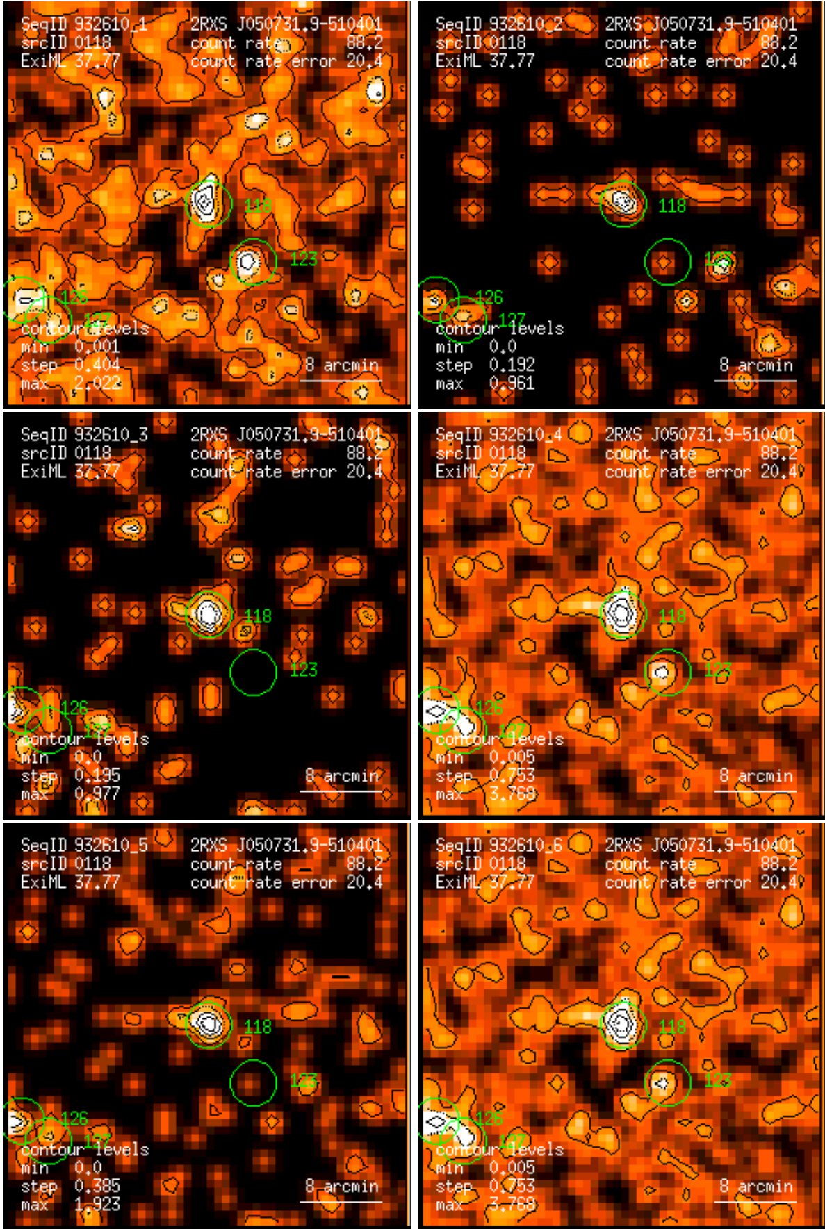
Figure 118: RASS 932610: detection 0118: band rate images, Gaussian filter: (1) PSPC channels 11 – 41, (2) 52 – 90, (3) 91 – 201, (4) 11 – 235, (5) 52 – 201, (6) 11 – 201. Broad band rates in counts/ks. Band rate contour levels in counts/ks/arcmin 2 .
