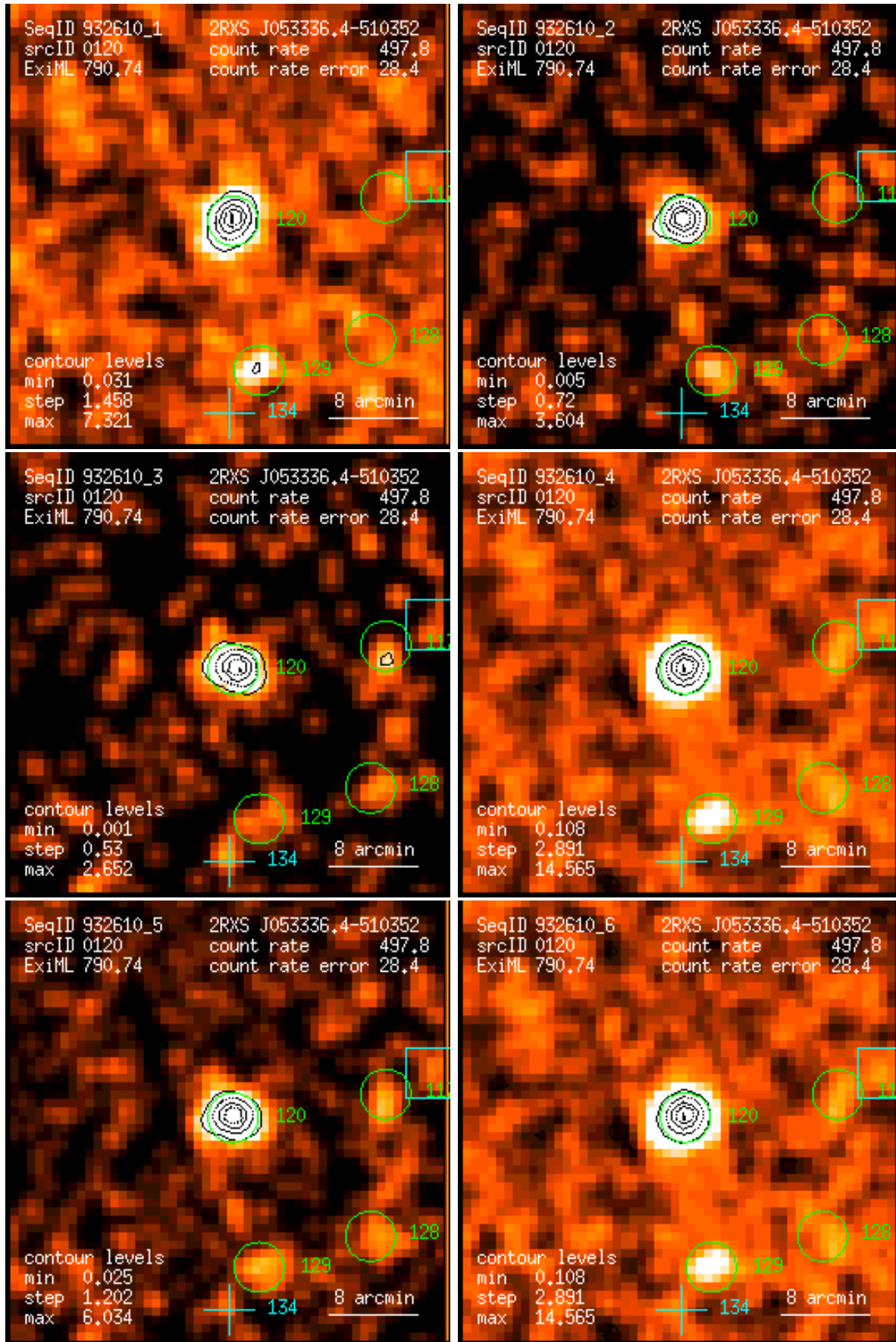
Figure 120: RASS 932610: detection 0120: band rate images, Gaussian filter: (1) PSPC channels 11 – 41, (2) 52 – 90, (3) 91 – 201, (4) 11 – 235, (5) 52 – 201, (6) 11 – 201. Broad band rates in counts/ks. Band rate contour levels in counts/ks/arcmin 2 .
