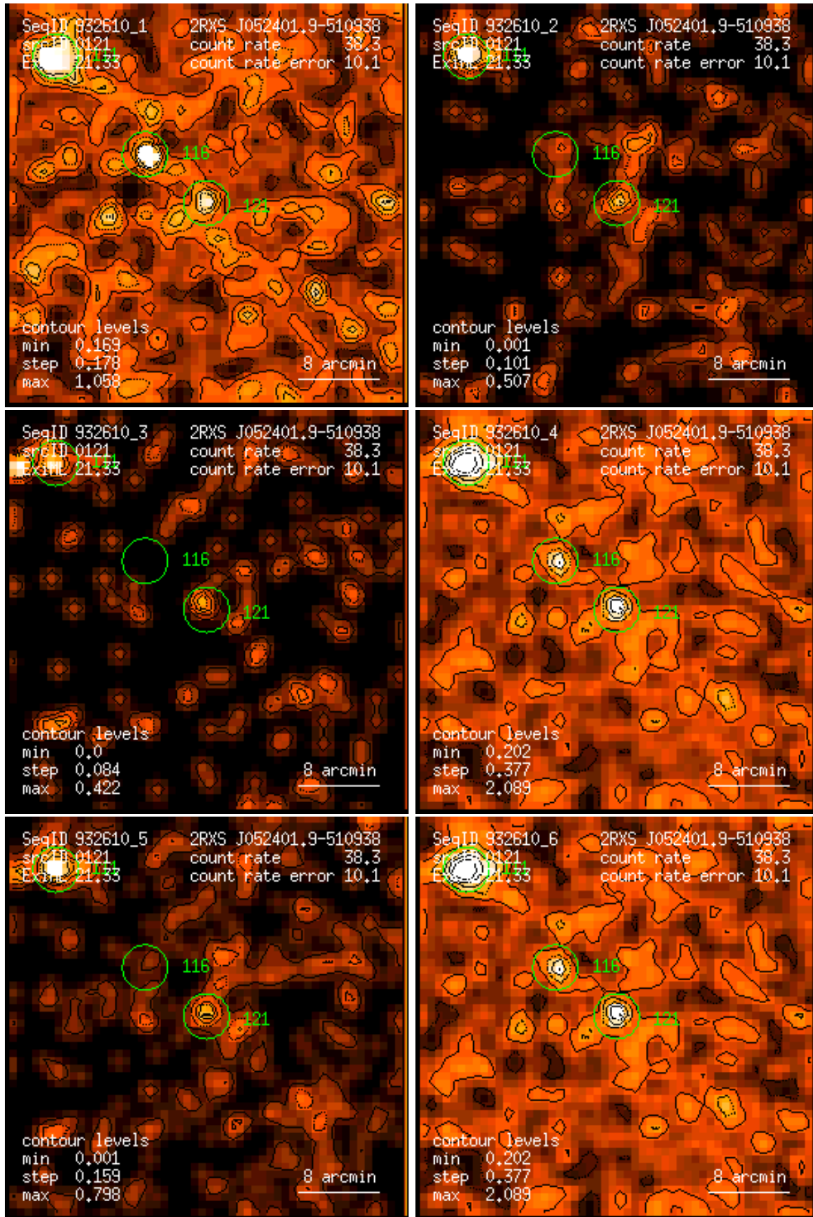
Figure 121: RASS 932610: detection 0121: band rate images, Gaussian filter: (1) PSPC channels 11 – 41, (2) 52 – 90, (3) 91 – 201, (4) 11 – 235, (5) 52 – 201, (6) 11 – 201. Broad band rates in counts/ks. Band rate contour levels in counts/ks/arcmin 2 .
