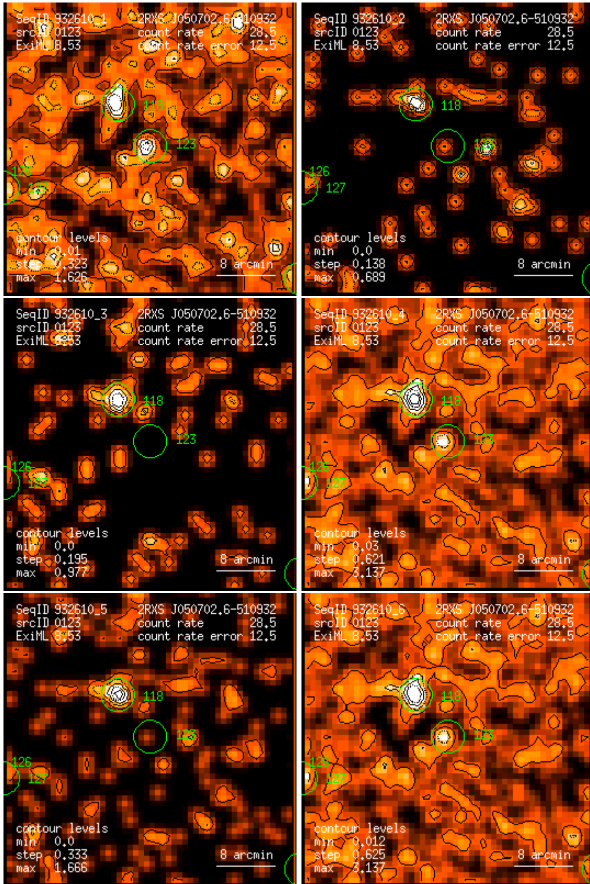
Figure 123: RASS 932610: detection 0123: band rate images, Gaussian filter: (1) PSPC channels 11 – 41, (2) 52 – 90, (3) 91 – 201, (4) 11 – 235, (5) 52 – 201, (6) 11 – 201. Broad band rates in counts/ks. Band rate contour levels in counts/ks/arcmin 2 .
