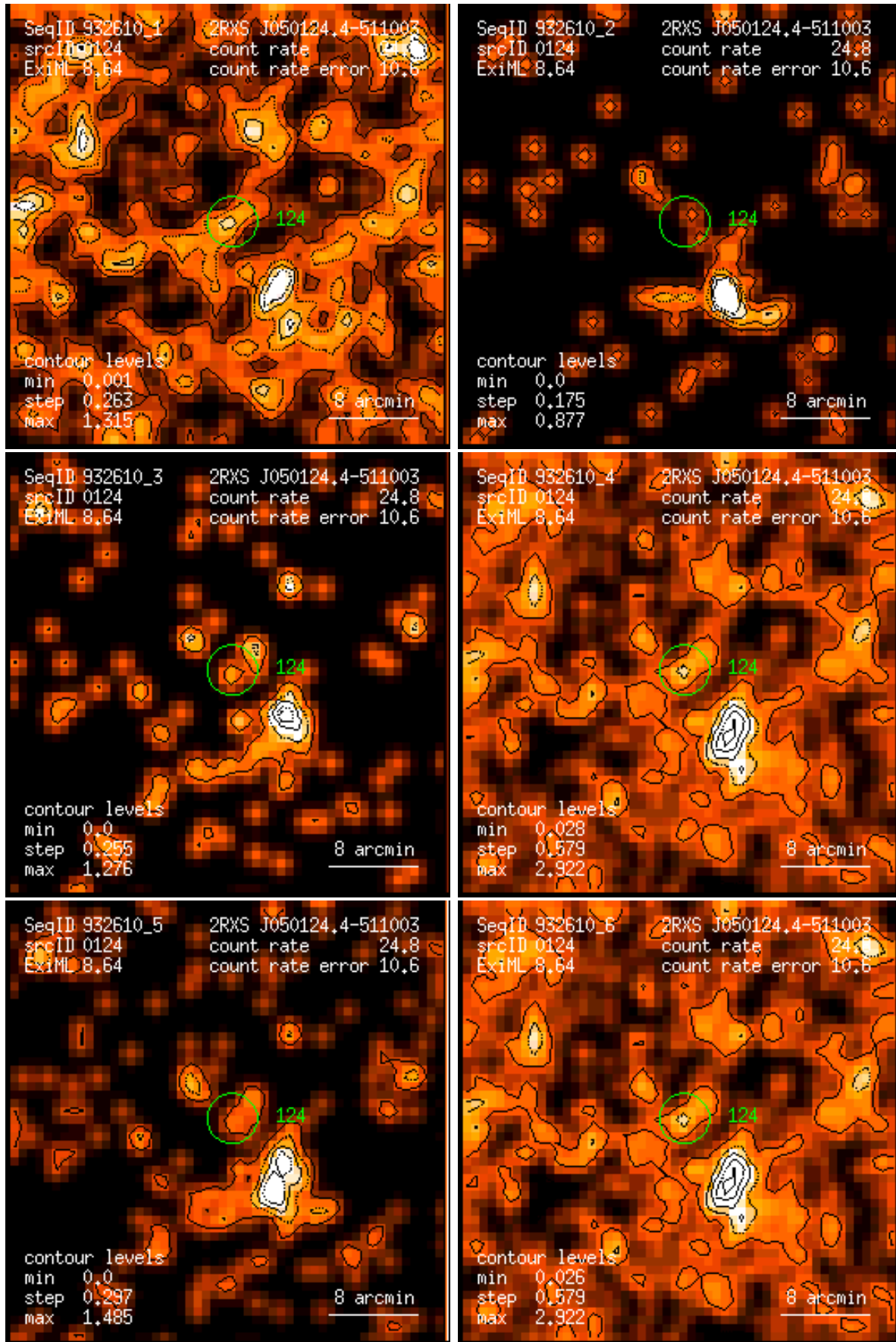
Figure 124: RASS 932610: detection 0124: band rate images, Gaussian filter: (1) PSPC channels 11 – 41, (2) 52 – 90, (3) 91 – 201, (4) 11 – 235, (5) 52 – 201, (6) 11 – 201. Broad band rates in counts/ks. Band rate contour levels in counts/ks/arcmin 2 .
