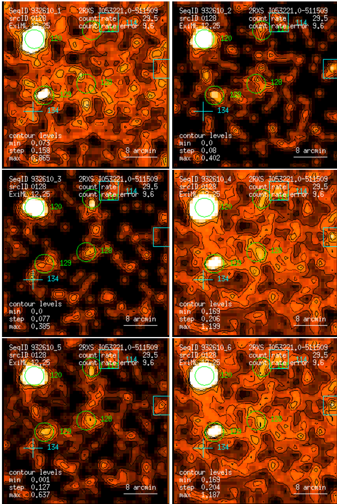
Figure 128: RASS 932610: detection 0128: band rate images, Gaussian filter: (1) PSPC channels 11 – 41, (2) 52 – 90, (3) 91 – 201, (4) 11 – 235, (5) 52 – 201, (6) 11 – 201. Broad band rates in counts/ks. Band rate contour levels in counts/ks/arcmin 2 .
