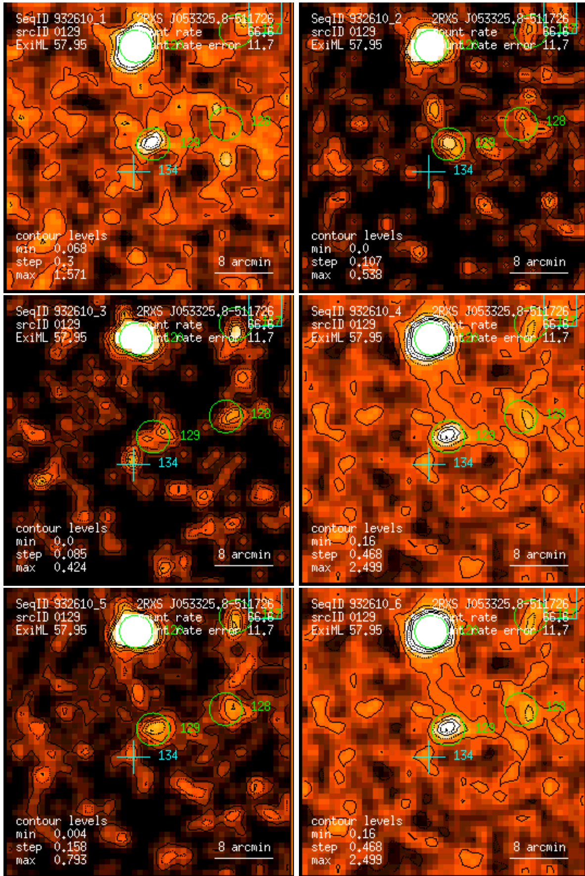
Figure 129: RASS 932610: detection 0129: band rate images, Gaussian filter: (1) PSPC channels 11 – 41, (2) 52 – 90, (3) 91 – 201, (4) 11 – 235, (5) 52 – 201, (6) 11 – 201. Broad band rates in counts/ks. Band rate contour levels in counts/ks/arcmin 2 .
