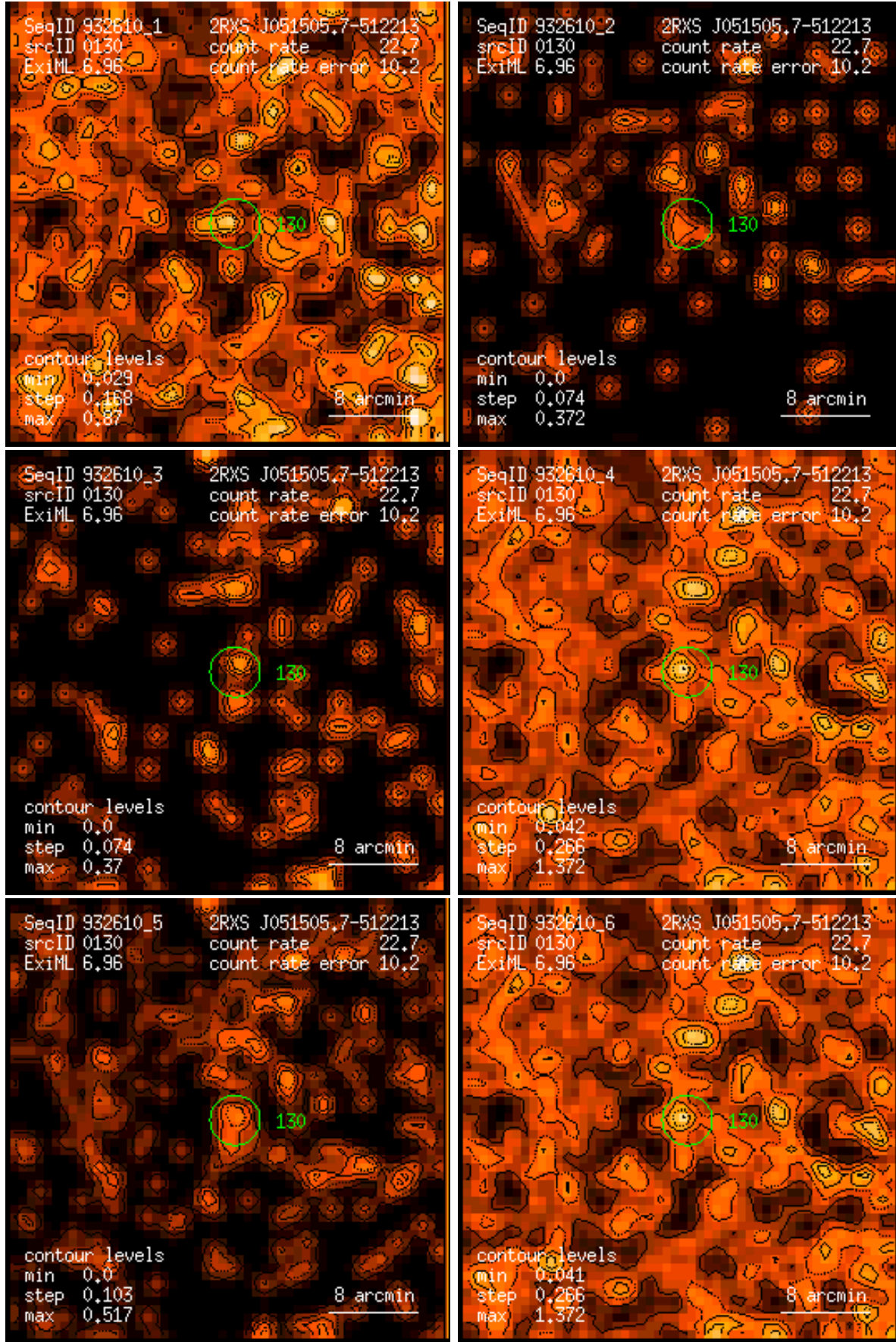
Figure 130: RASS 932610: detection 0130: band rate images, Gaussian filter: (1) PSPC channels 11 – 41, (2) 52 – 90, (3) 91 – 201, (4) 11 – 235, (5) 52 – 201, (6) 11 – 201. Broad band rates in counts/ks. Band rate contour levels in counts/ks/arcmin 2 .
