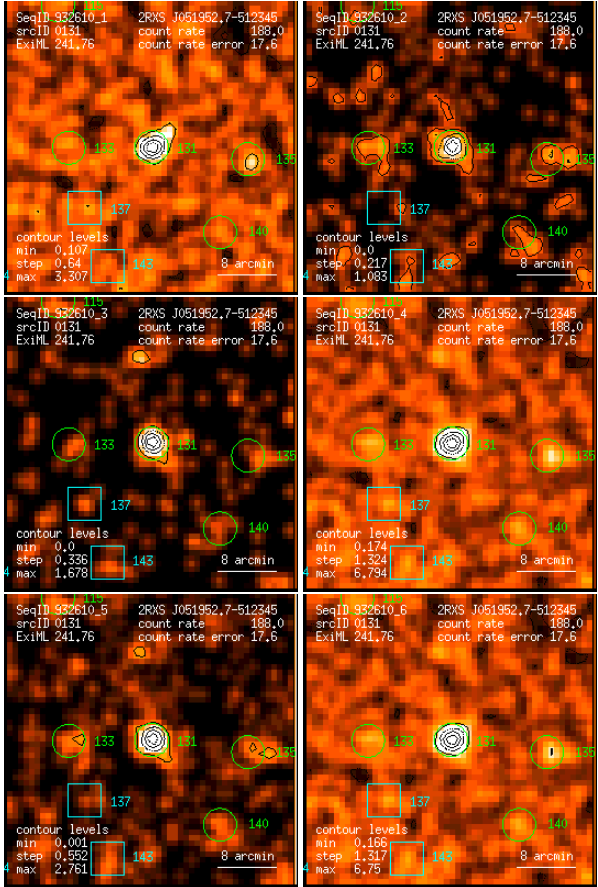
Figure 131: RASS 932610: detection 0131: band rate images, Gaussian filter: (1) PSPC channels 11 – 41, (2) 52 – 90, (3) 91 – 201, (4) 11 – 235, (5) 52 – 201, (6) 11 – 201. Broad band rates in counts/ks. Band rate contour levels in counts/ks/arcmin 2 .
