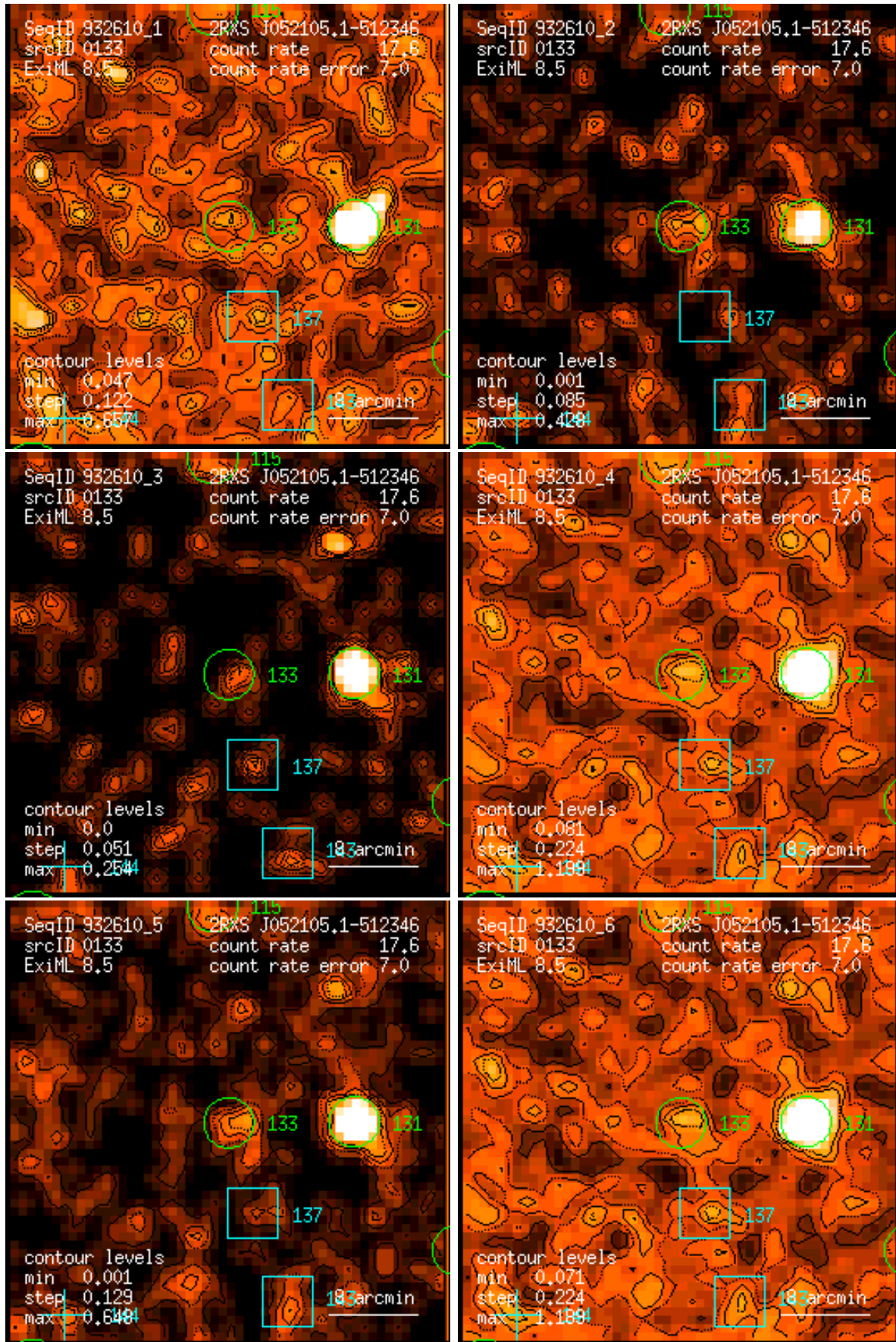
Figure 133: RASS 932610: detection 0133: band rate images, Gaussian filter: (1) PSPC channels 11 – 41, (2) 52 – 90, (3) 91 – 201, (4) 11 – 235, (5) 52 – 201, (6) 11 – 201. Broad band rates in counts/ks. Band rate contour levels in counts/ks/arcmin 2 .
