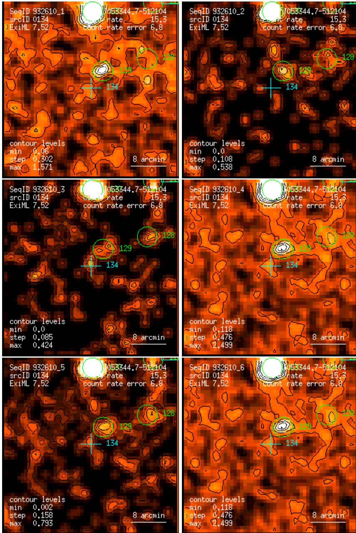
Figure 134: RASS 932610: detection 0134: band rate images, Gaussian filter: (1) PSPC channels 11 – 41, (2) 52 – 90, (3) 91 – 201, (4) 11 – 235, (5) 52 – 201, (6) 11 – 201. Broad band rates in counts/ks. Band rate contour levels in counts/ks/arcmin 2 .
