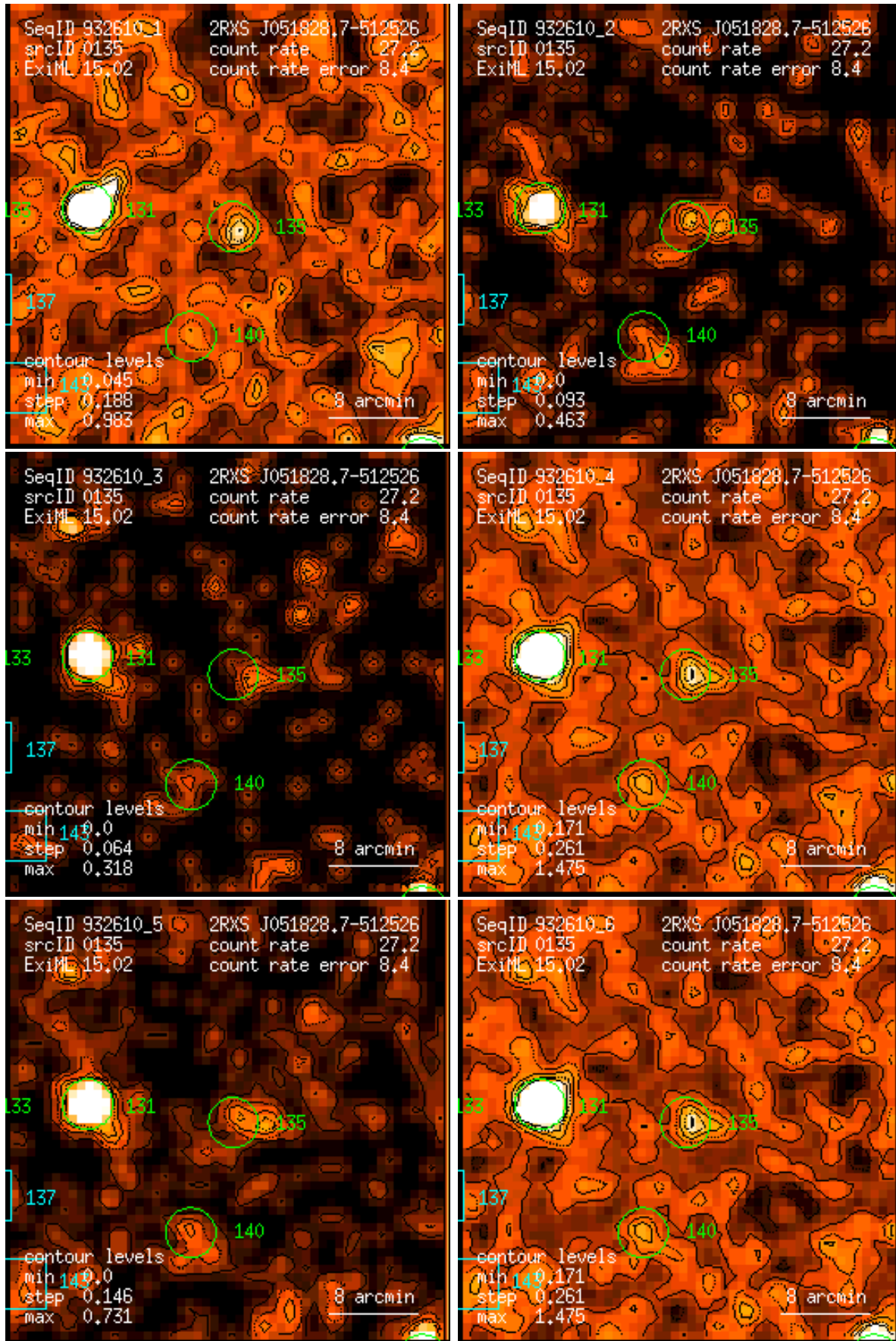
Figure 135: RASS 932610: detection 0135: band rate images, Gaussian filter: (1) PSPC channels 11 – 41, (2) 52 – 90, (3) 91 – 201, (4) 11 – 235, (5) 52 – 201, (6) 11 – 201. Broad band rates in counts/ks. Band rate contour levels in counts/ks/arcmin 2 .
