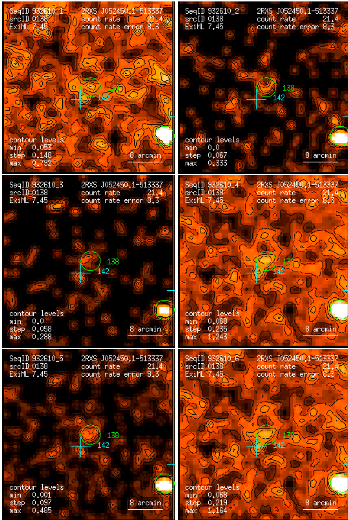
Figure 138: RASS 932610: detection 0138: band rate images, Gaussian filter: (1) PSPC channels 11 – 41, (2) 52 – 90, (3) 91 – 201, (4) 11 – 235, (5) 52 – 201, (6) 11 – 201. Broad band rates in counts/ks. Band rate contour levels in counts/ks/arcmin 2 .
