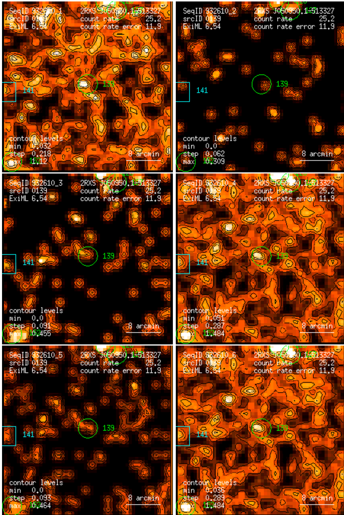
Figure 139: RASS 932610: detection 0139: band rate images, Gaussian filter: (1) PSPC channels 11 – 41, (2) 52 – 90, (3) 91 – 201, (4) 11 – 235, (5) 52 – 201, (6) 11 – 201. Broad band rates in counts/ks. Band rate contour levels in counts/ks/arcmin 2 .
