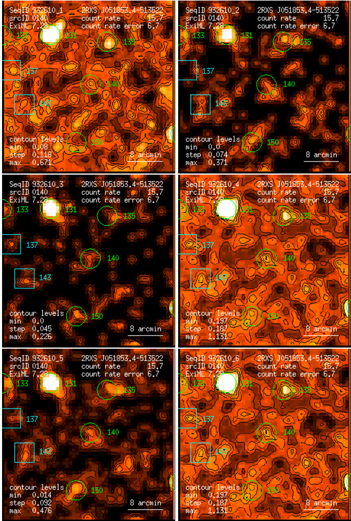
Figure 140: RASS 932610: detection 0140: band rate images, Gaussian filter: (1) PSPC channels 11 – 41, (2) 52 – 90, (3) 91 – 201, (4) 11 – 235, (5) 52 – 201, (6) 11 – 201. Broad band rates in counts/ks. Band rate contour levels in counts/ks/arcmin 2 .
