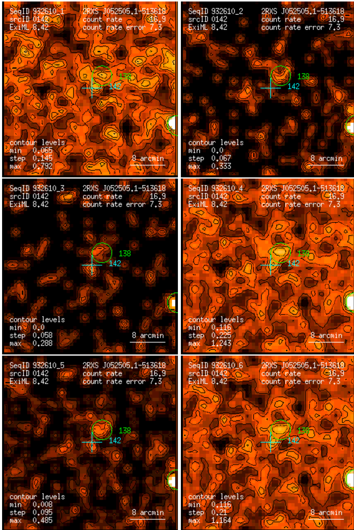
Figure 142: RASS 932610: detection 0142: band rate images, Gaussian filter: (1) PSPC channels 11 – 41, (2) 52 – 90, (3) 91 – 201, (4) 11 – 235, (5) 52 – 201, (6) 11 – 201. Broad band rates in counts/ks. Band rate contour levels in counts/ks/arcmin 2 .
