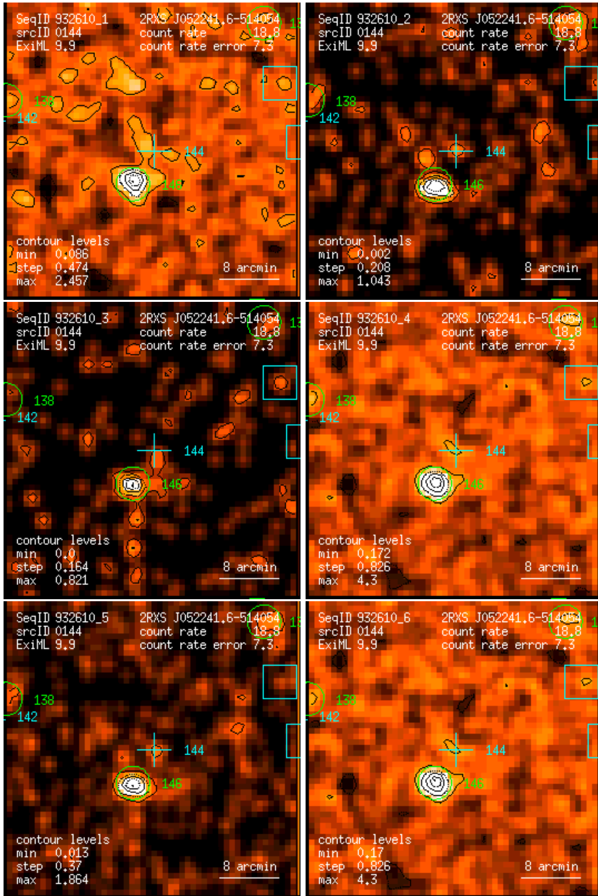
Figure 144: RASS 932610: detection 0144: band rate images, Gaussian filter: (1) PSPC channels 11 – 41, (2) 52 – 90, (3) 91 – 201, (4) 11 – 235, (5) 52 – 201, (6) 11 – 201. Broad band rates in counts/ks. Band rate contour levels in counts/ks/arcmin 2 .
