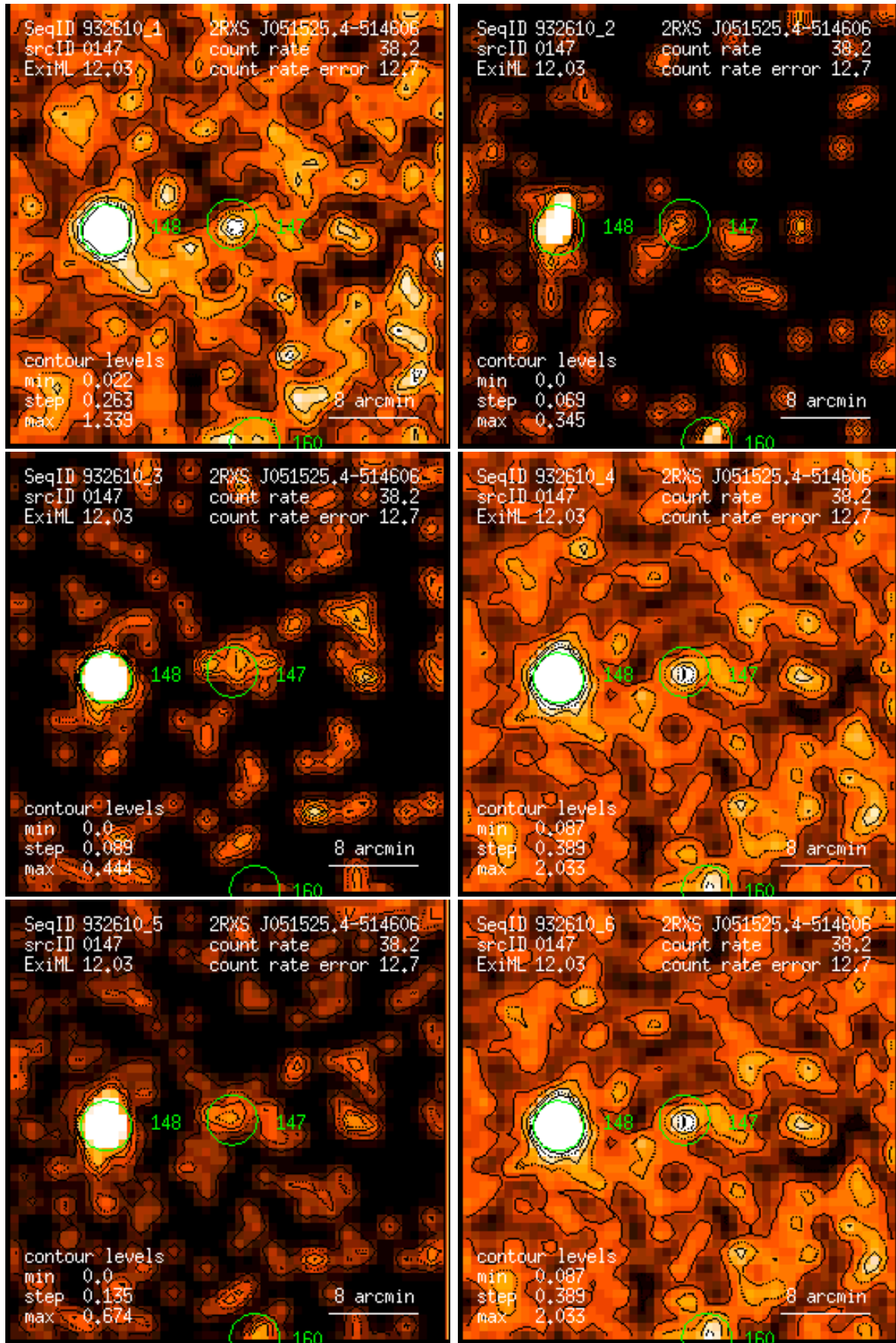
Figure 147: RASS 932610: detection 0147: band rate images, Gaussian filter: (1) PSPC channels 11 – 41, (2) 52 – 90, (3) 91 – 201, (4) 11 – 235, (5) 52 – 201, (6) 11 – 201. Broad band rates in counts/ks. Band rate contour levels in counts/ks/arcmin 2 .
