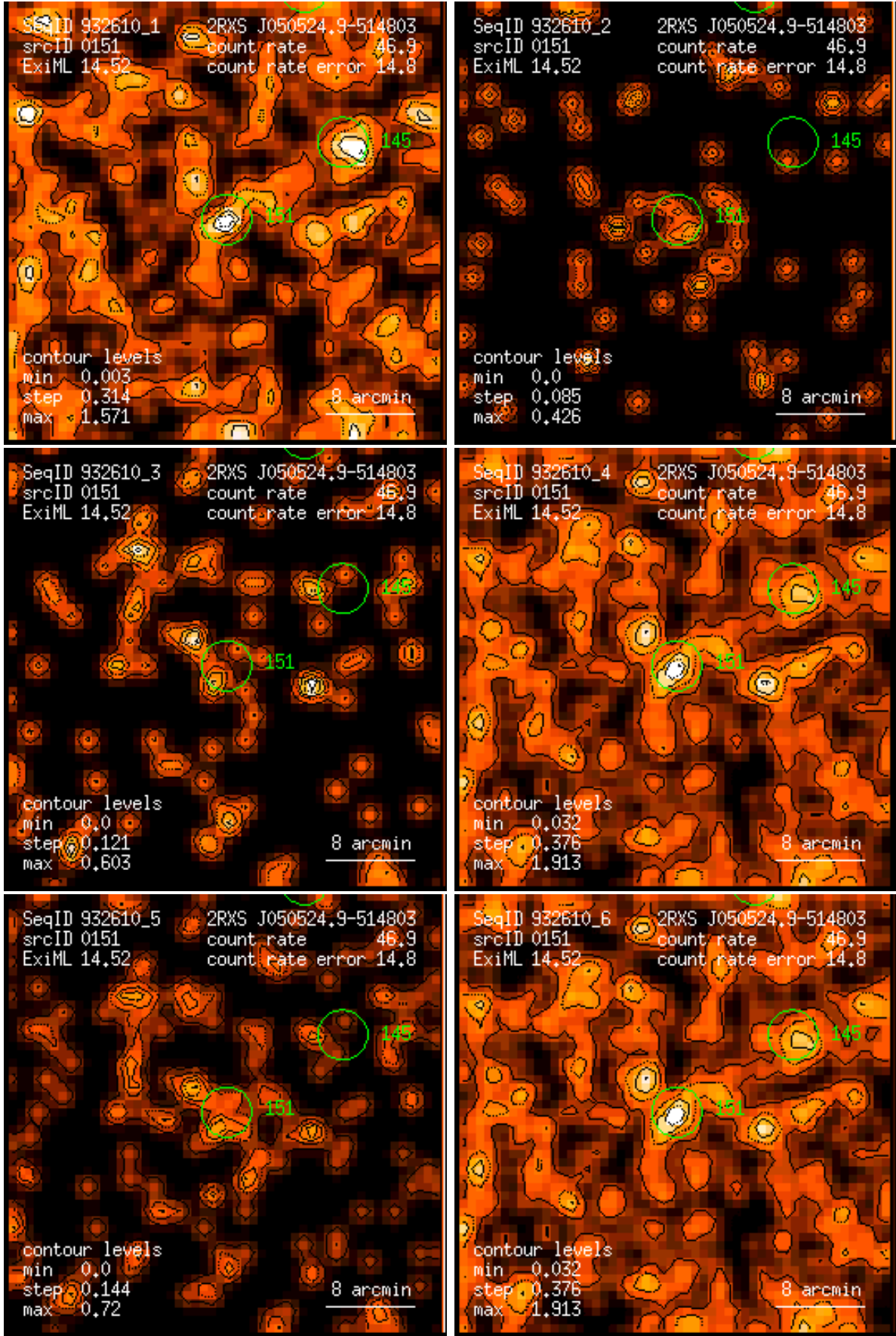
Figure 151: RASS 932610: detection 0151: band rate images, Gaussian filter: (1) PSPC channels 11 – 41, (2) 52 – 90, (3) 91 – 201, (4) 11 – 235, (5) 52 – 201, (6) 11 – 201. Broad band rates in counts/ks. Band rate contour levels in counts/ks/arcmin 2 .
