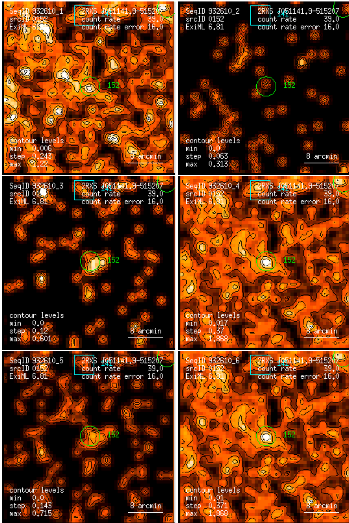
Figure 152: RASS 932610: detection 0152: band rate images, Gaussian filter: (1) PSPC channels 11 – 41, (2) 52 – 90, (3) 91 – 201, (4) 11 – 235, (5) 52 – 201, (6) 11 – 201. Broad band rates in counts/ks. Band rate contour levels in counts/ks/arcmin 2 .
