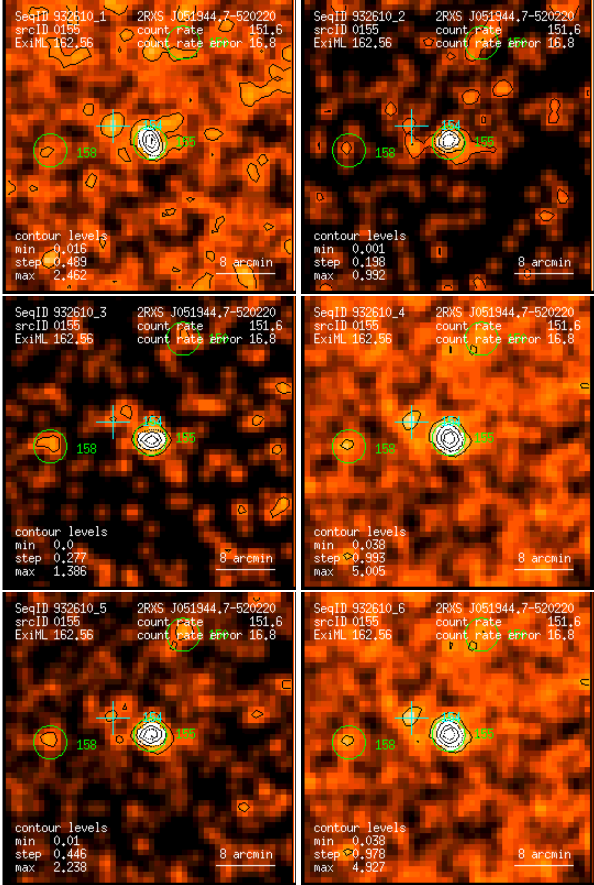
Figure 155: RASS 932610: detection 0155: band rate images, Gaussian filter: (1) PSPC channels 11 – 41, (2) 52 – 90, (3) 91 – 201, (4) 11 – 235, (5) 52 – 201, (6) 11 – 201. Broad band rates in counts/ks. Band rate contour levels in counts/ks/arcmin 2 .
