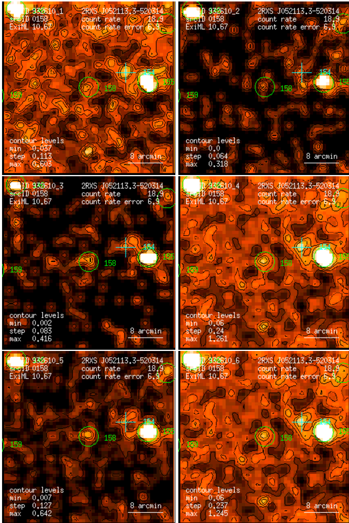
Figure 158: RASS 932610: detection 0158: band rate images, Gaussian filter: (1) PSPC channels 11 – 41, (2) 52 – 90, (3) 91 – 201, (4) 11 – 235, (5) 52 – 201, (6) 11 – 201. Broad band rates in counts/ks. Band rate contour levels in counts/ks/arcmin 2 .
