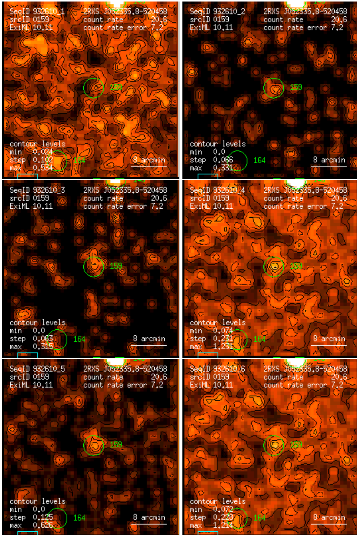
Figure 159: RASS 932610: detection 0159: band rate images, Gaussian filter: (1) PSPC channels 11 – 41, (2) 52 – 90, (3) 91 – 201, (4) 11 – 235, (5) 52 – 201, (6) 11 – 201. Broad band rates in counts/ks. Band rate contour levels in counts/ks/arcmin 2 .
