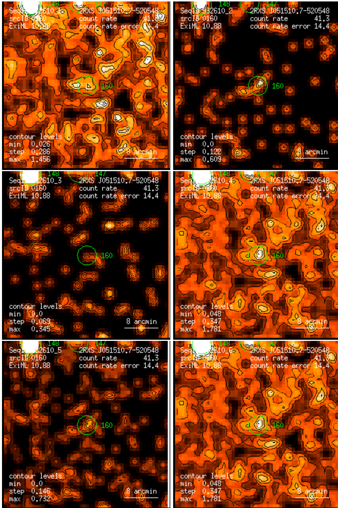
Figure 160: RASS 932610: detection 0160: band rate images, Gaussian filter: (1) PSPC channels 11 – 41, (2) 52 – 90, (3) 91 – 201, (4) 11 – 235, (5) 52 – 201, (6) 11 – 201. Broad band rates in counts/ks. Band rate contour levels in counts/ks/arcmin 2 .
