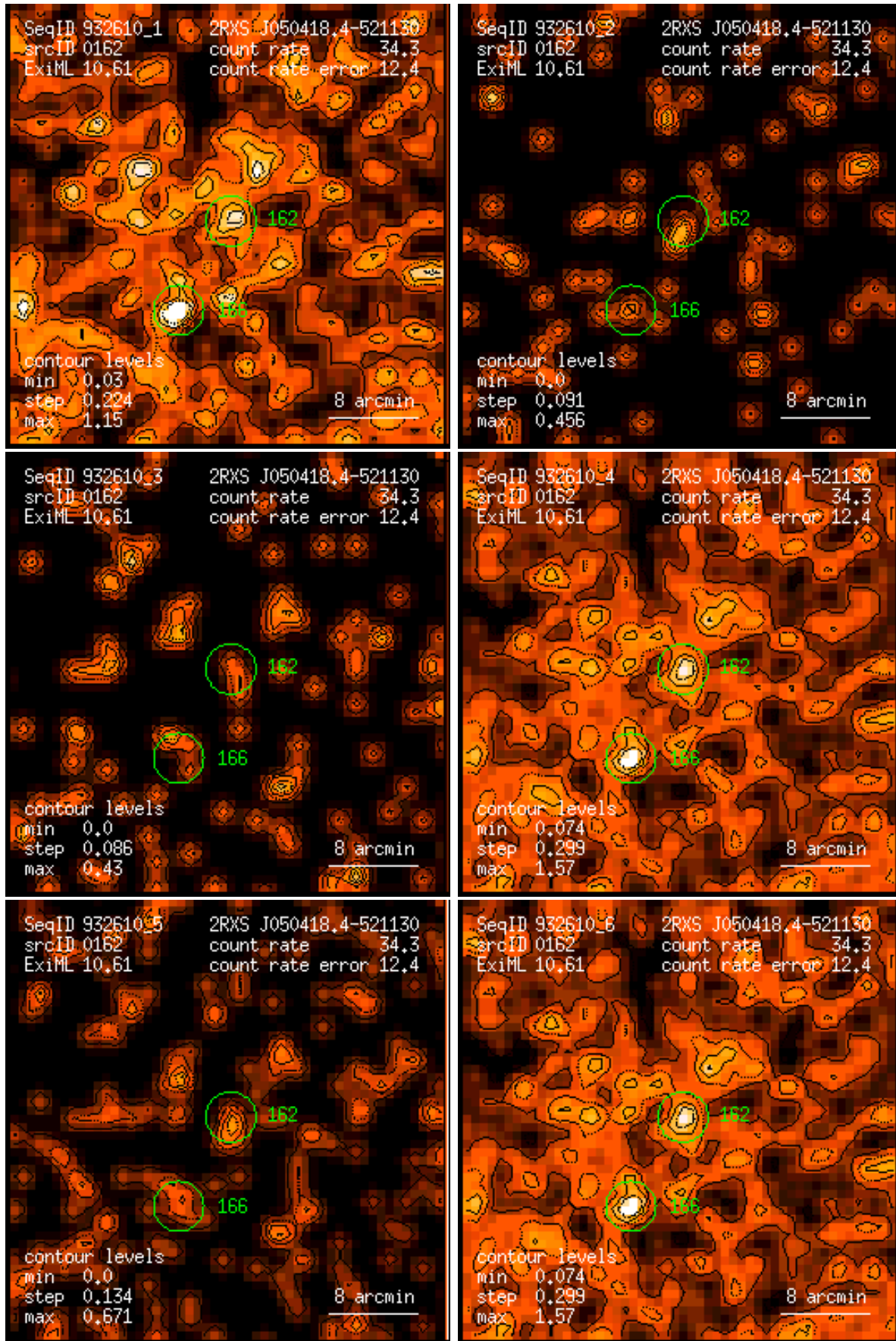
Figure 162: RASS 932610: detection 0162: band rate images, Gaussian filter: (1) PSPC channels 11 – 41, (2) 52 – 90, (3) 91 – 201, (4) 11 – 235, (5) 52 – 201, (6) 11 – 201. Broad band rates in counts/ks. Band rate contour levels in counts/ks/arcmin 2 .
