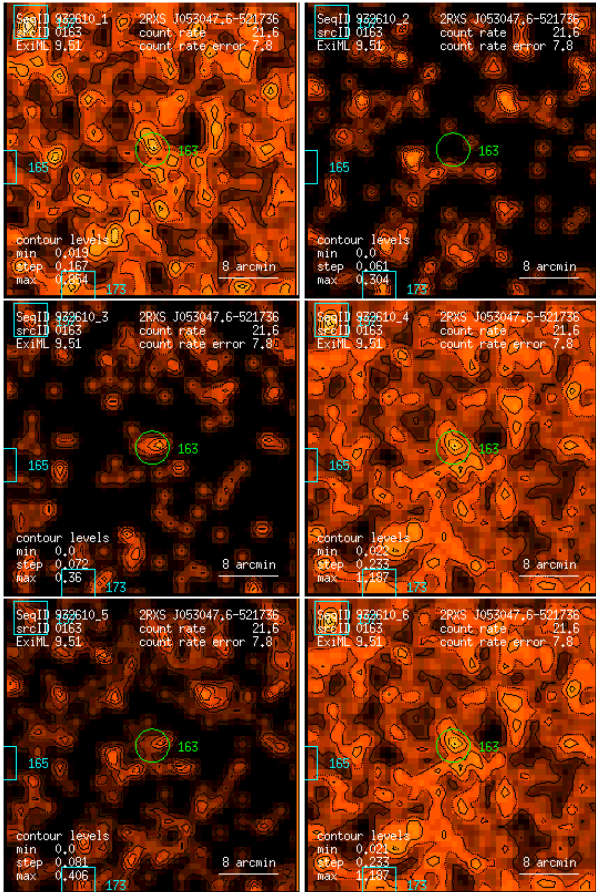
Figure 163: RASS 932610: detection 0163: band rate images, Gaussian filter: (1) PSPC channels 11 – 41, (2) 52 – 90, (3) 91 – 201, (4) 11 – 235, (5) 52 – 201, (6) 11 – 201. Broad band rates in counts/ks. Band rate contour levels in counts/ks/arcmin 2 .
