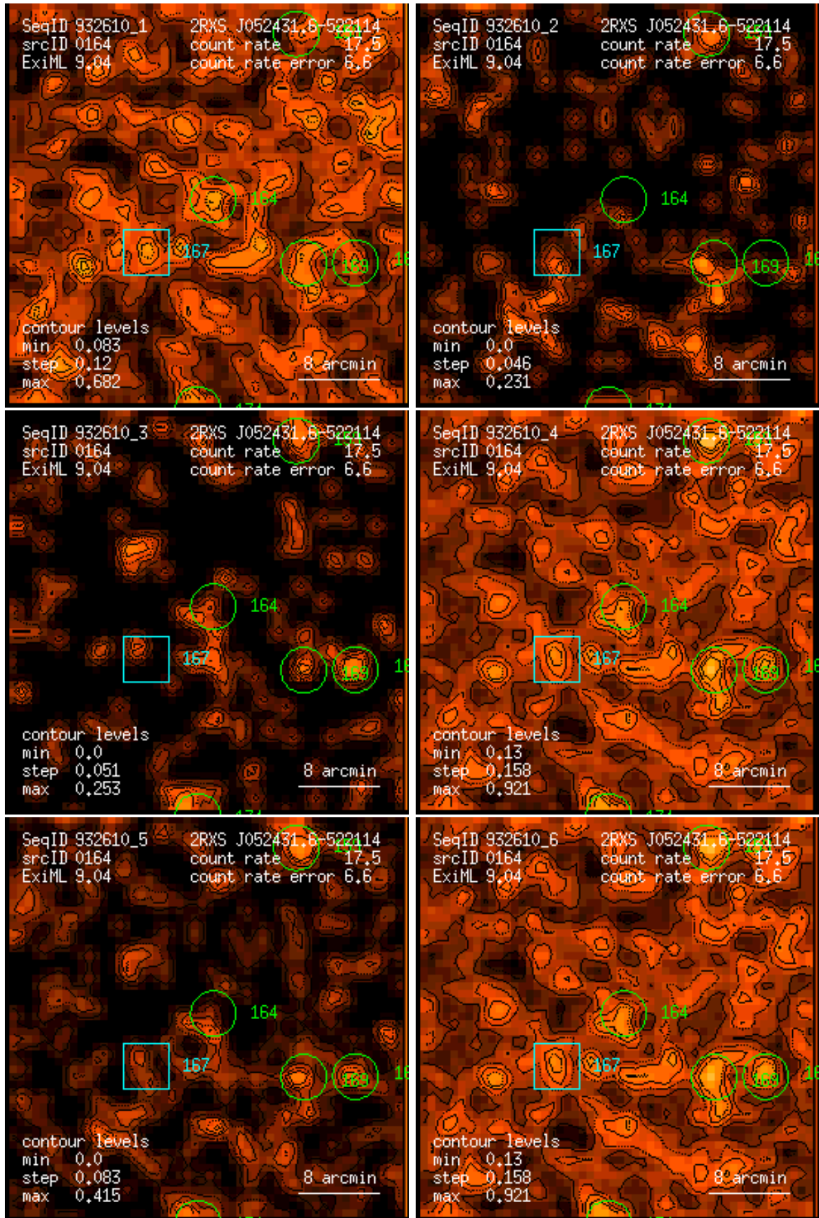
Figure 164: RASS 932610: detection 0164: band rate images, Gaussian filter: (1) PSPC channels 11 – 41, (2) 52 – 90, (3) 91 – 201, (4) 11 – 235, (5) 52 – 201, (6) 11 – 201. Broad band rates in counts/ks. Band rate contour levels in counts/ks/arcmin 2 .
