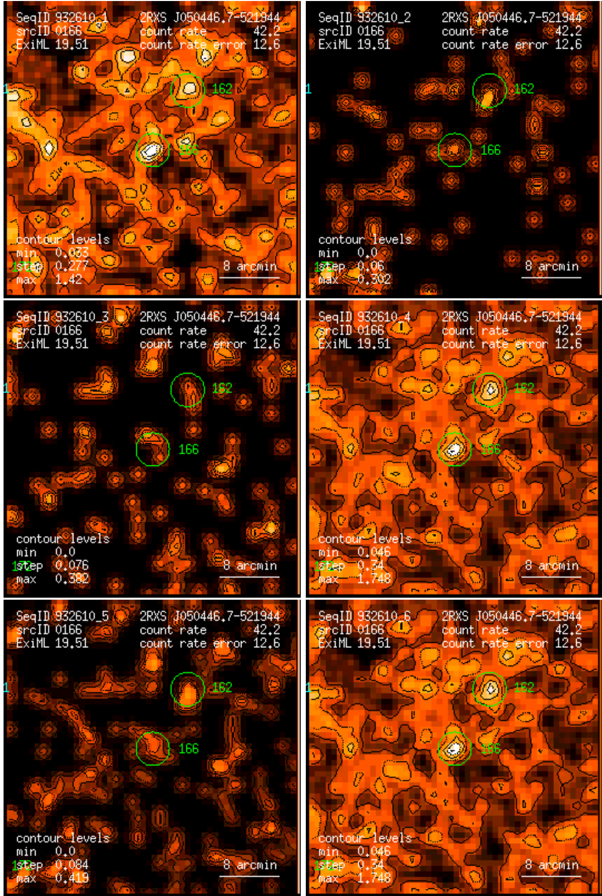
Figure 166: RASS 932610: detection 0166: band rate images, Gaussian filter: (1) PSPC channels 11 – 41, (2) 52 – 90, (3) 91 – 201, (4) 11 – 235, (5) 52 – 201, (6) 11 – 201. Broad band rates in counts/ks. Band rate contour levels in counts/ks/arcmin 2 .
