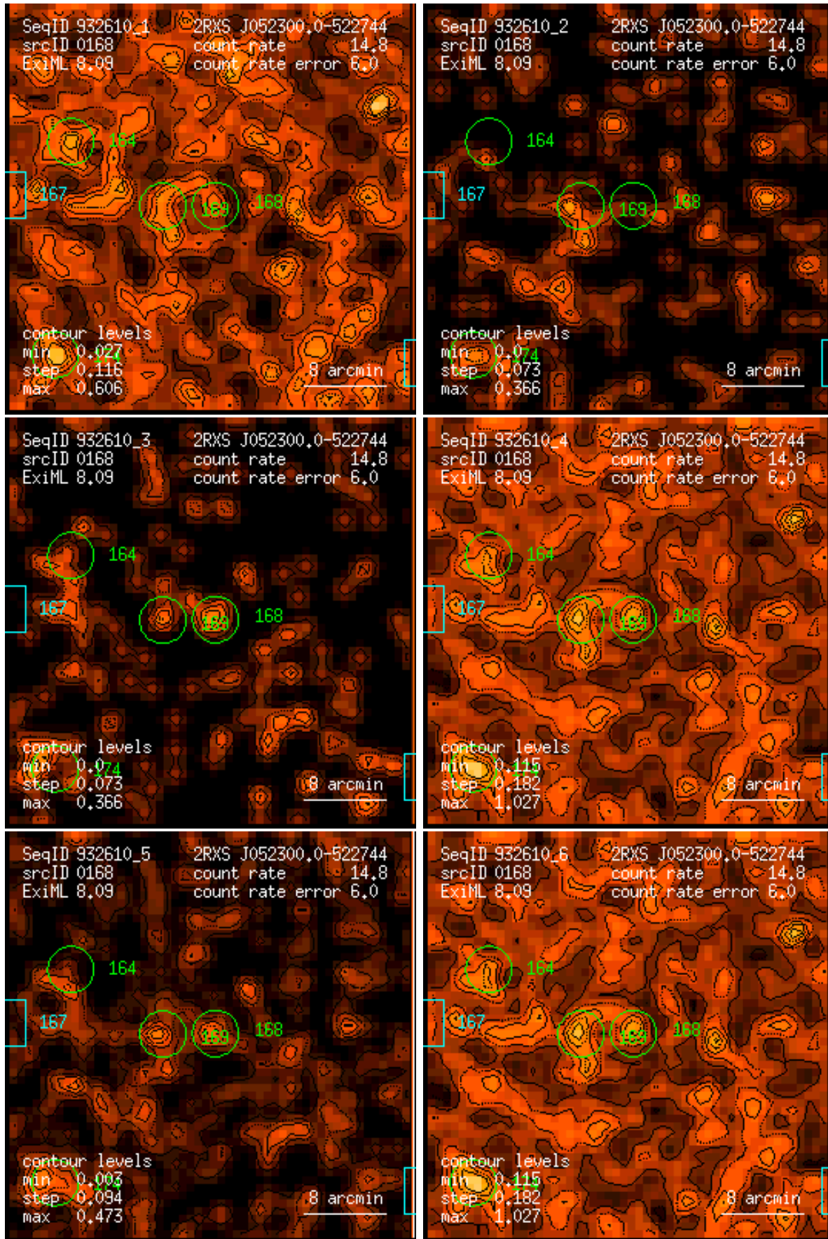
Figure 168: RASS 932610: detection 0168: band rate images, Gaussian filter: (1) PSPC channels 11 – 41, (2) 52 – 90, (3) 91 – 201, (4) 11 – 235, (5) 52 – 201, (6) 11 – 201. Broad band rates in counts/ks. Band rate contour levels in counts/ks/arcmin 2 .
