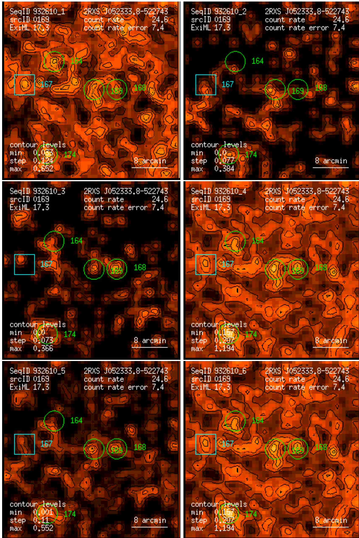
Figure 169: RASS 932610: detection 0169: band rate images, Gaussian filter: (1) PSPC channels 11 – 41, (2) 52 – 90, (3) 91 – 201, (4) 11 – 235, (5) 52 – 201, (6) 11 – 201. Broad band rates in counts/ks. Band rate contour levels in counts/ks/arcmin 2 .
