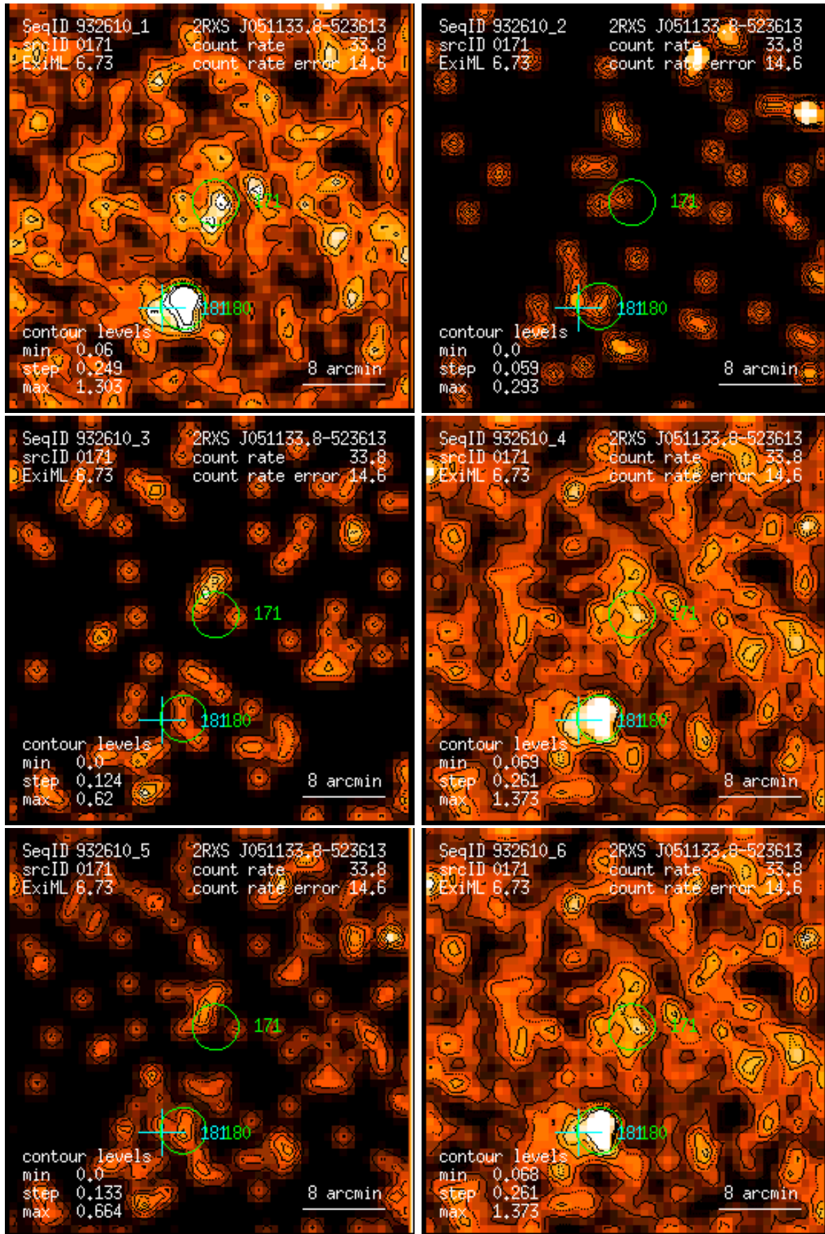
Figure 171: RASS 932610: detection 0171: band rate images, Gaussian filter: (1) PSPC channels 11 – 41, (2) 52 – 90, (3) 91 – 201, (4) 11 – 235, (5) 52 – 201, (6) 11 – 201. Broad band rates in counts/ks. Band rate contour levels in counts/ks/arcmin 2 .
