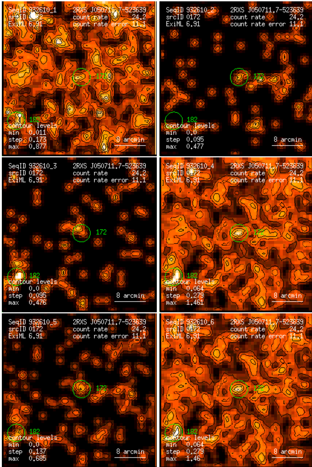
Figure 172: RASS 932610: detection 0172: band rate images, Gaussian filter: (1) PSPC channels 11 – 41, (2) 52 – 90, (3) 91 – 201, (4) 11 – 235, (5) 52 – 201, (6) 11 – 201. Broad band rates in counts/ks. Band rate contour levels in counts/ks/arcmin 2 .
