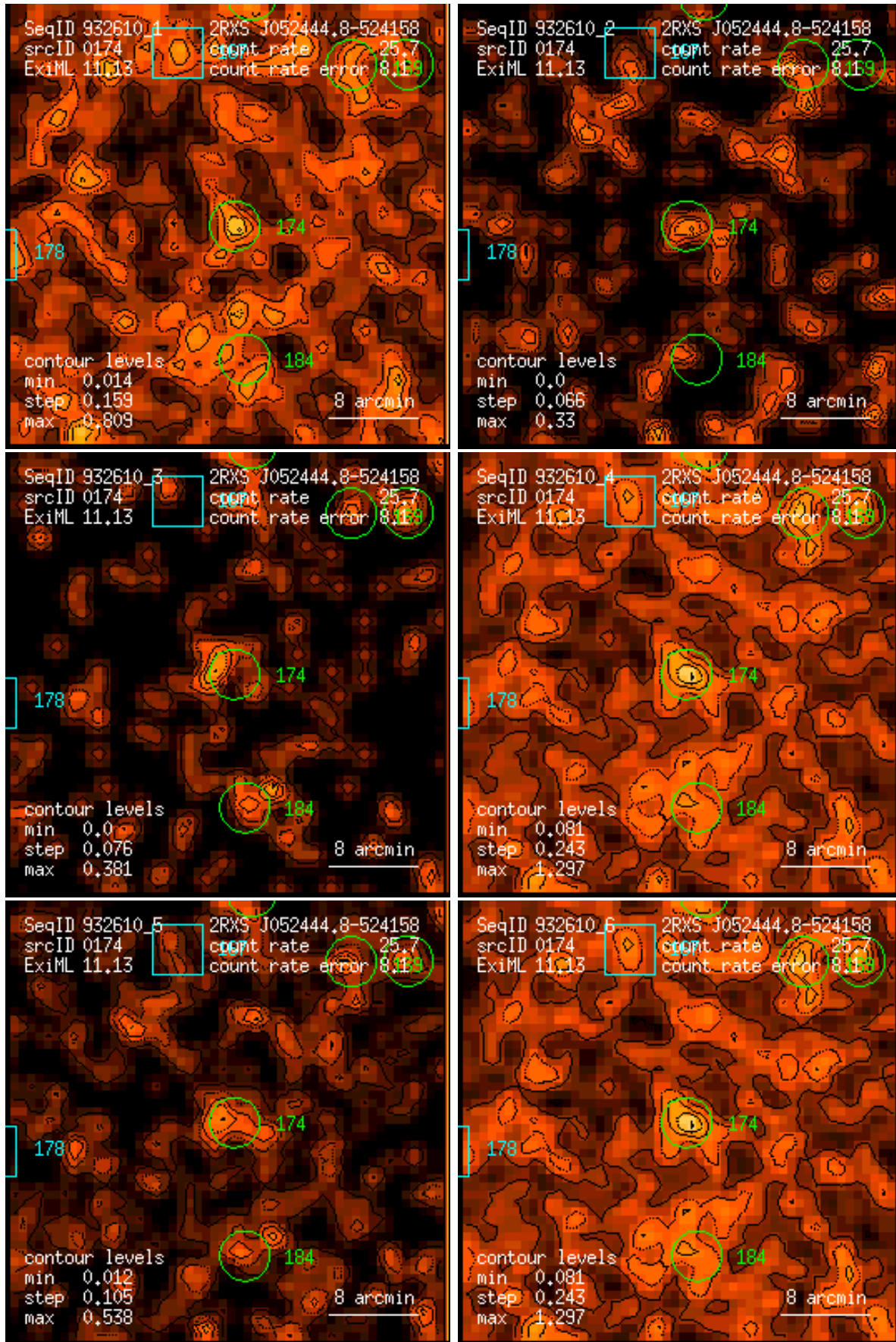
Figure 174: RASS 932610: detection 0174: band rate images, Gaussian filter: (1) PSPC channels 11 – 41, (2) 52 – 90, (3) 91 – 201, (4) 11 – 235, (5) 52 – 201, (6) 11 – 201. Broad band rates in counts/ks. Band rate contour levels in counts/ks/arcmin 2 .
