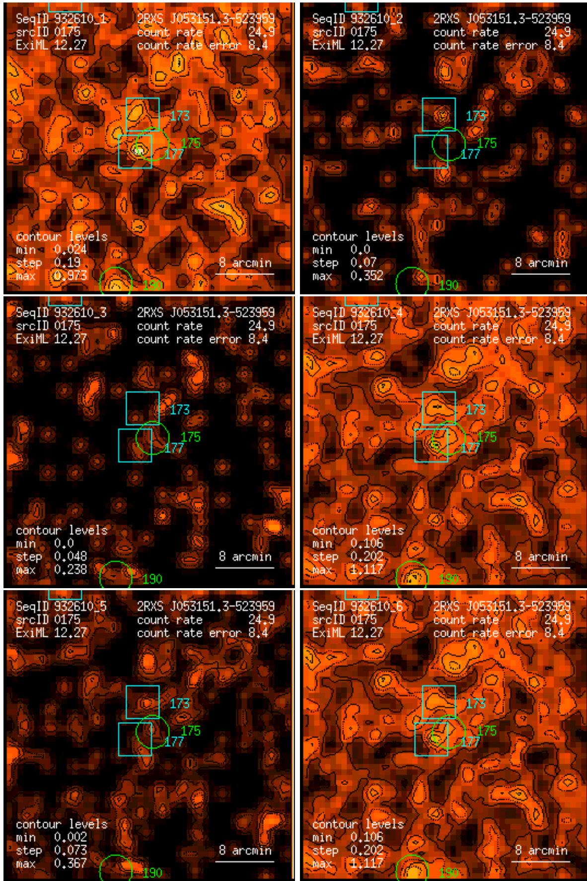
Figure 175: RASS 932610: detection 0175: band rate images, Gaussian filter: (1) PSPC channels 11 – 41, (2) 52 – 90, (3) 91 – 201, (4) 11 – 235, (5) 52 – 201, (6) 11 – 201. Broad band rates in counts/ks. Band rate contour levels in counts/ks/arcmin 2 .
