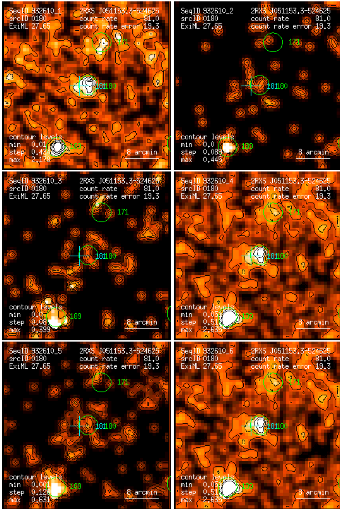
Figure 180: RASS 932610: detection 0180: band rate images, Gaussian filter: (1) PSPC channels 11 – 41, (2) 52 – 90, (3) 91 – 201, (4) 11 – 235, (5) 52 – 201, (6) 11 – 201. Broad band rates in counts/ks. Band rate contour levels in counts/ks/arcmin 2 .
