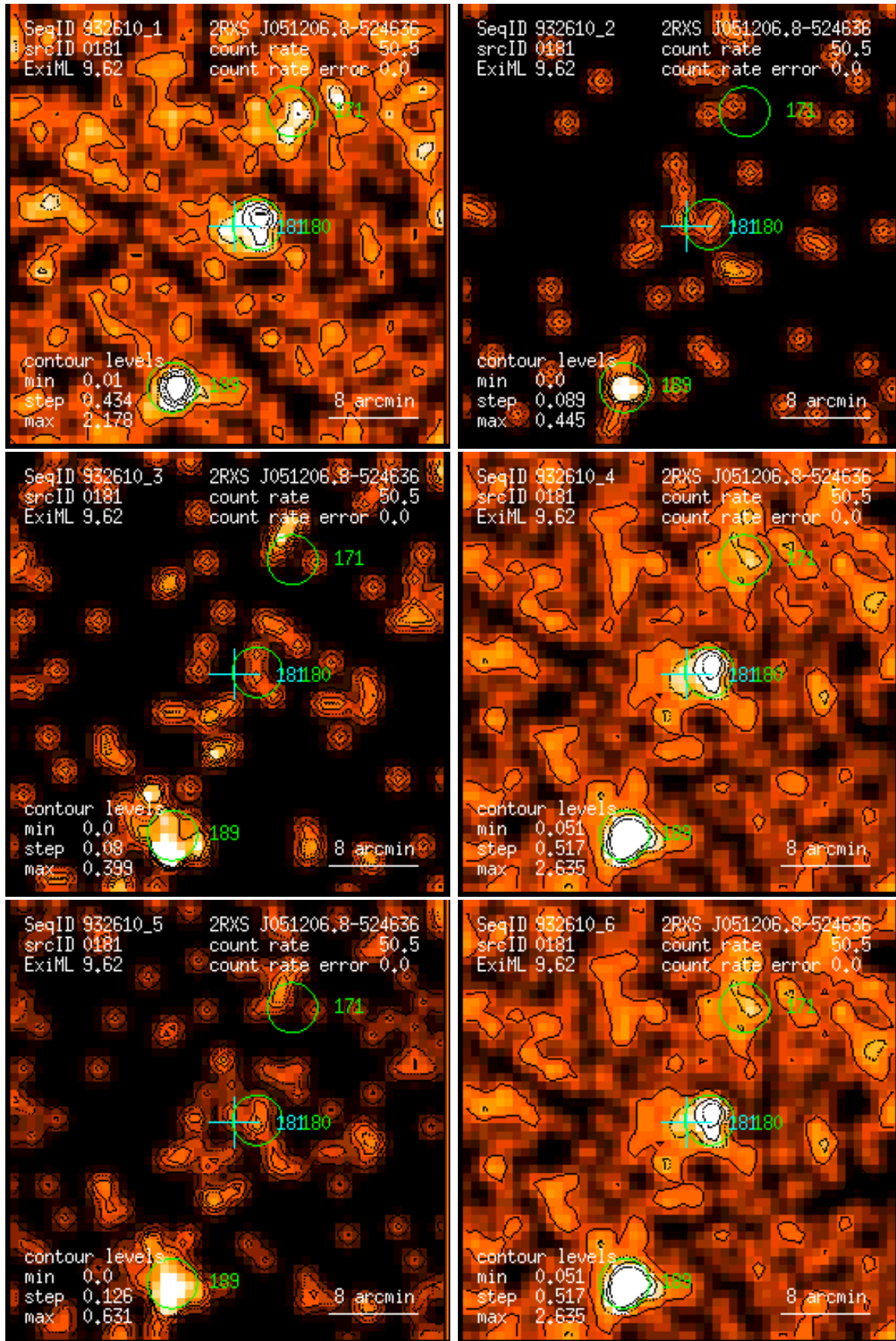
Figure 181: RASS 932610: detection 0181: band rate images, Gaussian filter: (1) PSPC channels 11 – 41, (2) 52 – 90, (3) 91 – 201, (4) 11 – 235, (5) 52 – 201, (6) 11 – 201. Broad band rates in counts/ks. Band rate contour levels in counts/ks/arcmin 2 .
