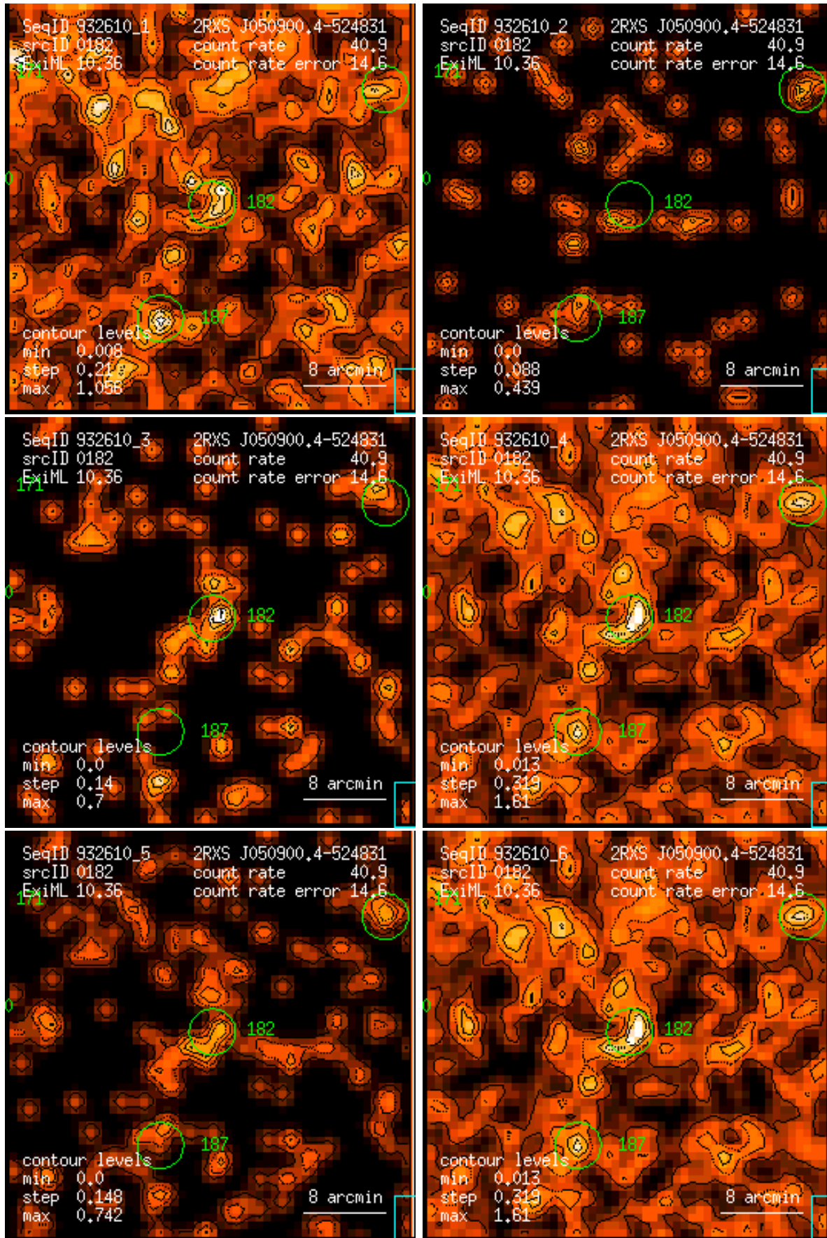
Figure 182: RASS 932610: detection 0182: band rate images, Gaussian filter: (1) PSPC channels 11 – 41, (2) 52 – 90, (3) 91 – 201, (4) 11 – 235, (5) 52 – 201, (6) 11 – 201. Broad band rates in counts/ks. Band rate contour levels in counts/ks/arcmin 2 .
