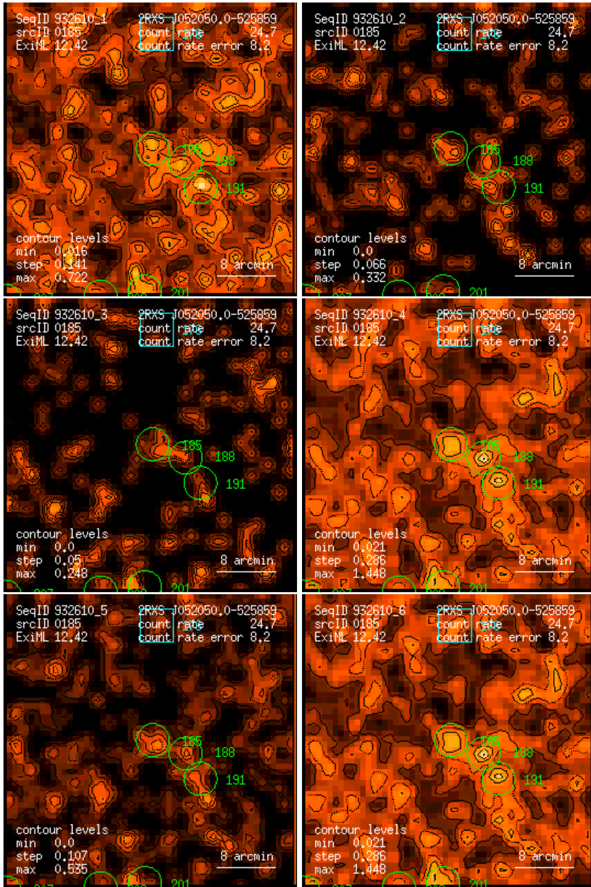
Figure 185: RASS 932610: detection 0185: band rate images, Gaussian filter: (1) PSPC channels 11 – 41, (2) 52 – 90, (3) 91 – 201, (4) 11 – 235, (5) 52 – 201, (6) 11 – 201. Broad band rates in counts/ks. Band rate contour levels in counts/ks/arcmin 2 .
