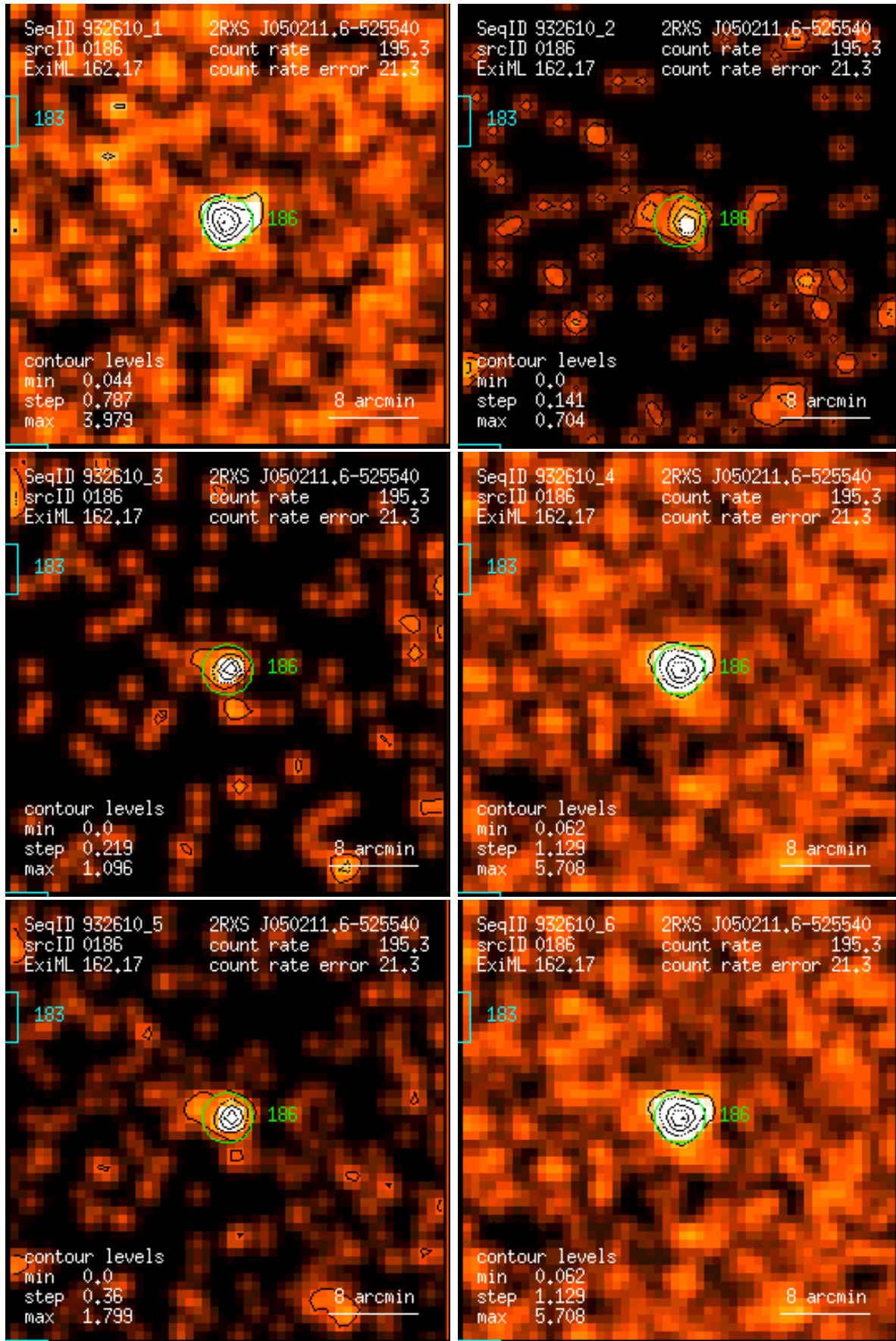
Figure 186: RASS 932610: detection 0186: band rate images, Gaussian filter: (1) PSPC channels 11 – 41, (2) 52 – 90, (3) 91 – 201, (4) 11 – 235, (5) 52 – 201, (6) 11 – 201. Broad band rates in counts/ks. Band rate contour levels in counts/ks/arcmin 2 .
