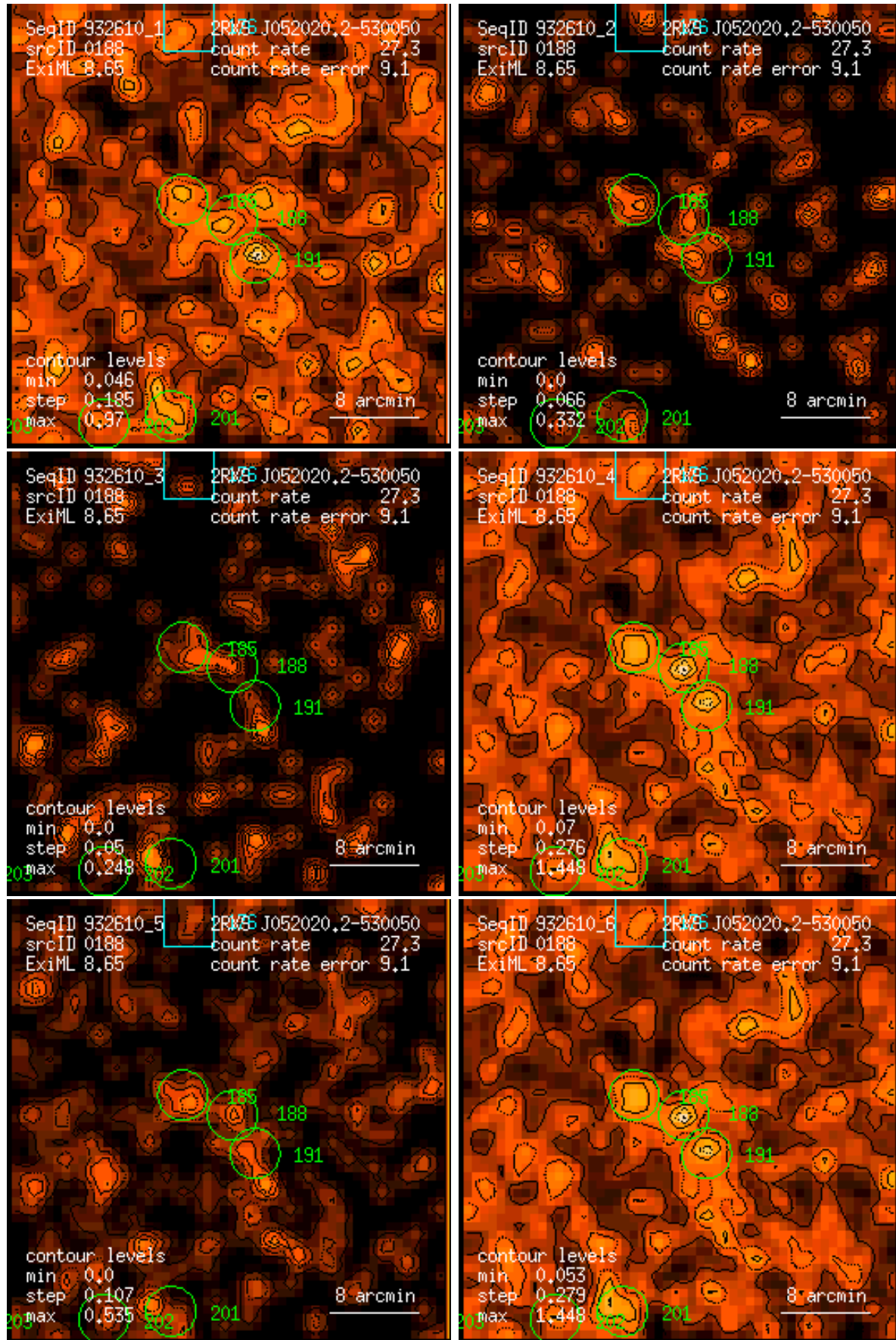
Figure 188: RASS 932610: detection 0188: band rate images, Gaussian filter: (1) PSPC channels 11 – 41, (2) 52 – 90, (3) 91 – 201, (4) 11 – 235, (5) 52 – 201, (6) 11 – 201. Broad band rates in counts/ks. Band rate contour levels in counts/ks/arcmin 2 .
