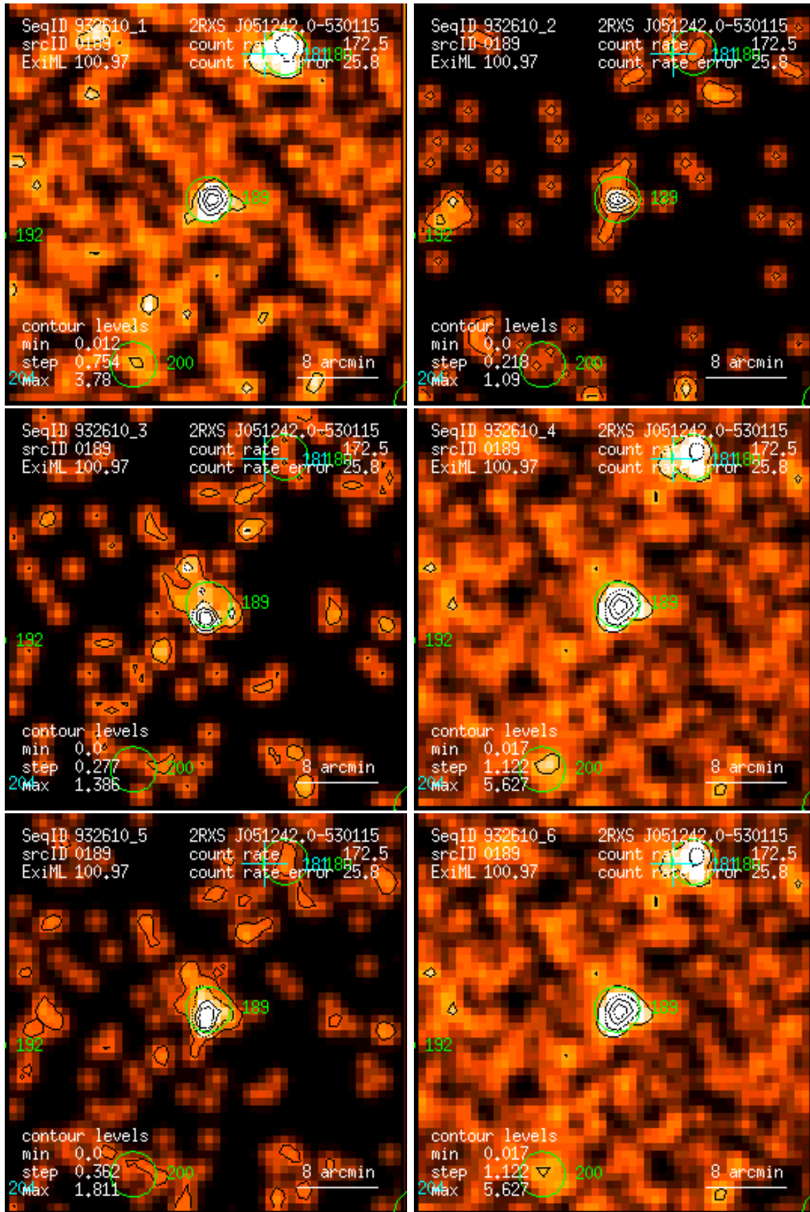
Figure 189: RASS 932610: detection 0189: band rate images, Gaussian filter: (1) PSPC channels 11 – 41, (2) 52 – 90, (3) 91 – 201, (4) 11 – 235, (5) 52 – 201, (6) 11 – 201. Broad band rates in counts/ks. Band rate contour levels in counts/ks/arcmin 2 .
