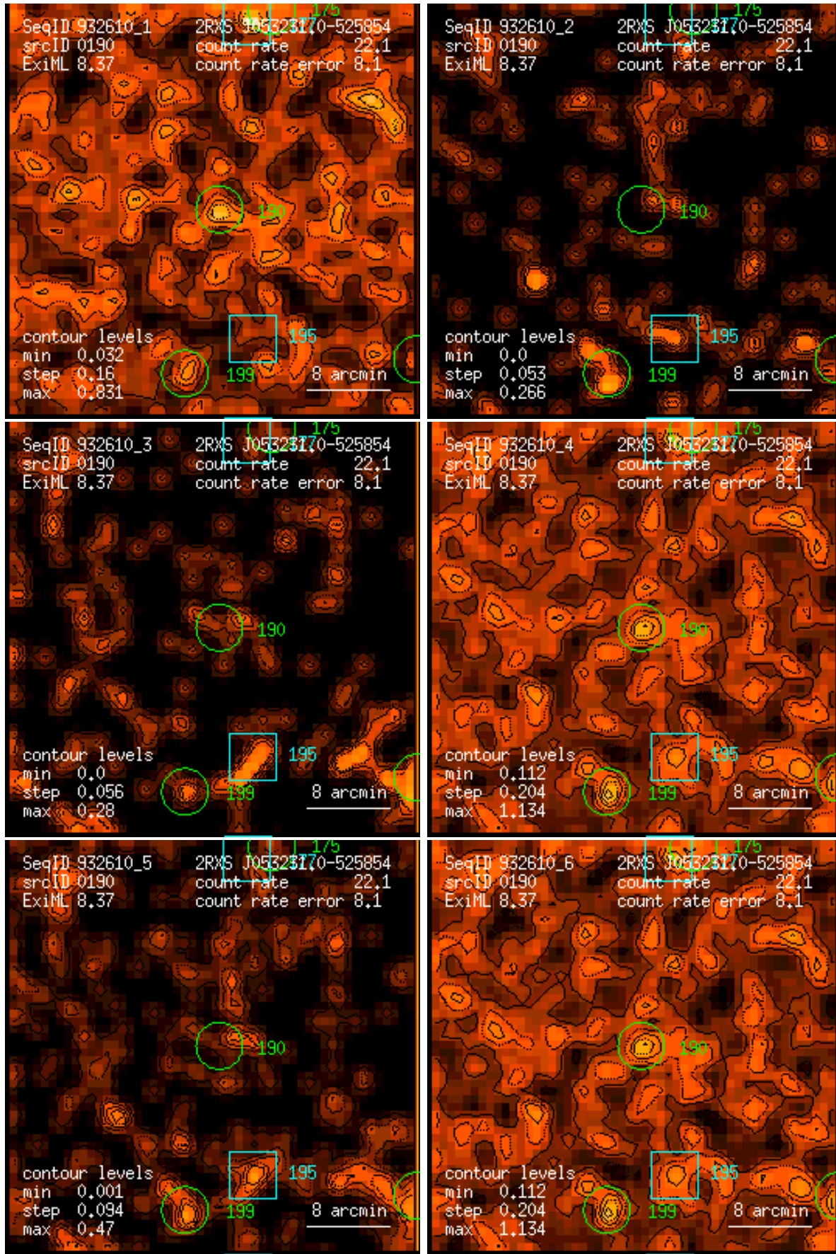
Figure 190: RASS 932610: detection 0190: band rate images, Gaussian filter: (1) PSPC channels 11 – 41, (2) 52 – 90, (3) 91 – 201, (4) 11 – 235, (5) 52 – 201, (6) 11 – 201. Broad band rates in counts/ks. Band rate contour levels in counts/ks/arcmin 2 .
